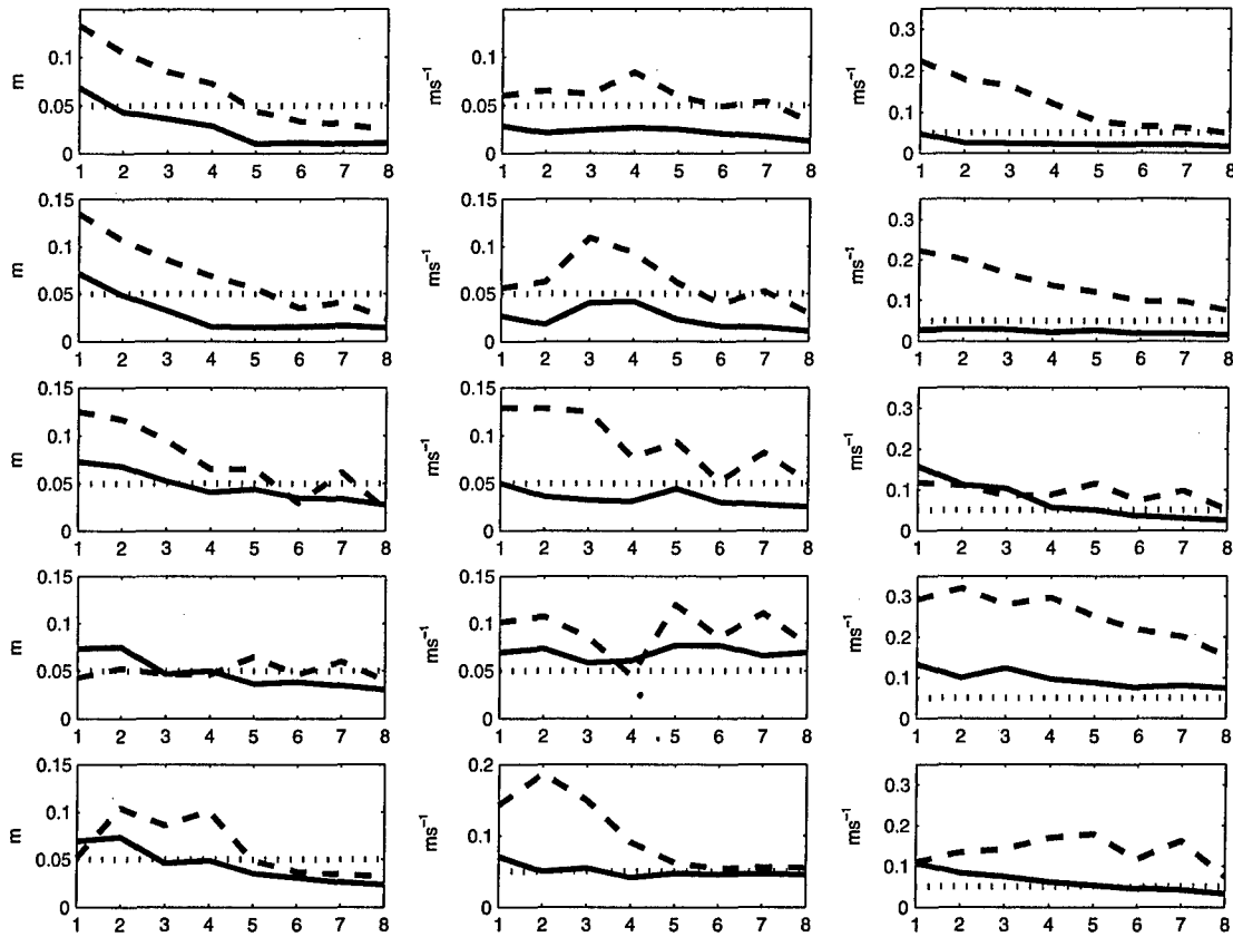
Fig. 5. This analysis is the same as Fig. 4 except the rms errors are computed over the entire assimilation window. Only the representer (solid line) and EnKS (dashed line) results are shown. The EnKF does not correct the initial condition, and thus is not comparable to the EnKS and representer solutions over the entire assimilation window.
