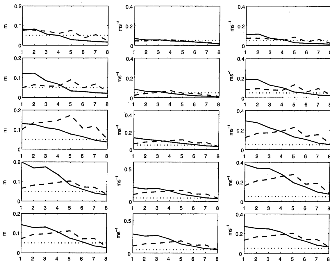
Fig. 10. The forecast rms error for the representer (solid line) and the EnKS/EnKF (dashed line), with all data assimilated. The dotted line is the measurement noise level, and the x-axis is the network number.
