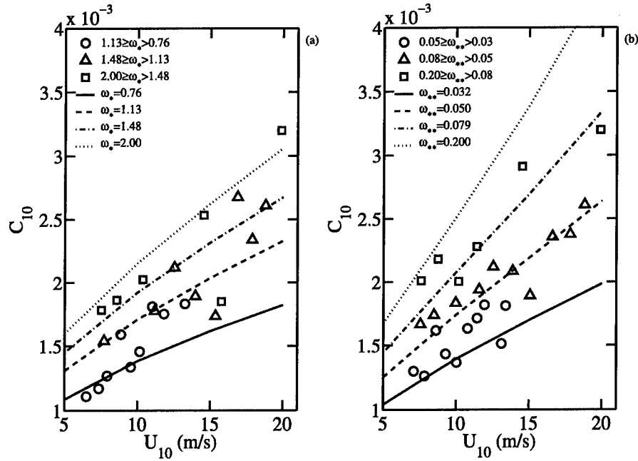
Figure 3. (a) C_{10} calculated using equation (7) and presented as a function of U_{10} ; (b) same as Figure 3a, but C_{10} is calculated using equation (1). The DMAJ data are superimposed for comparison.
