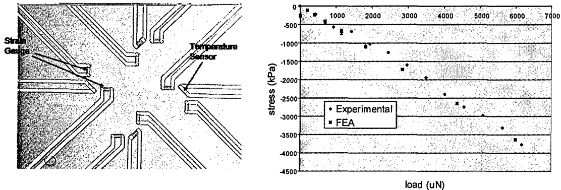
Figure 19. Embedded strain sensors (left) and match with data from our coating theoretical models (right). Note that the sensors are underneath the coatings and are thus do not impact the mirror's interaction with the light. The experimental plot shown is film stress as a function of mechanical load. The modeling has been performed using finite element methods.
