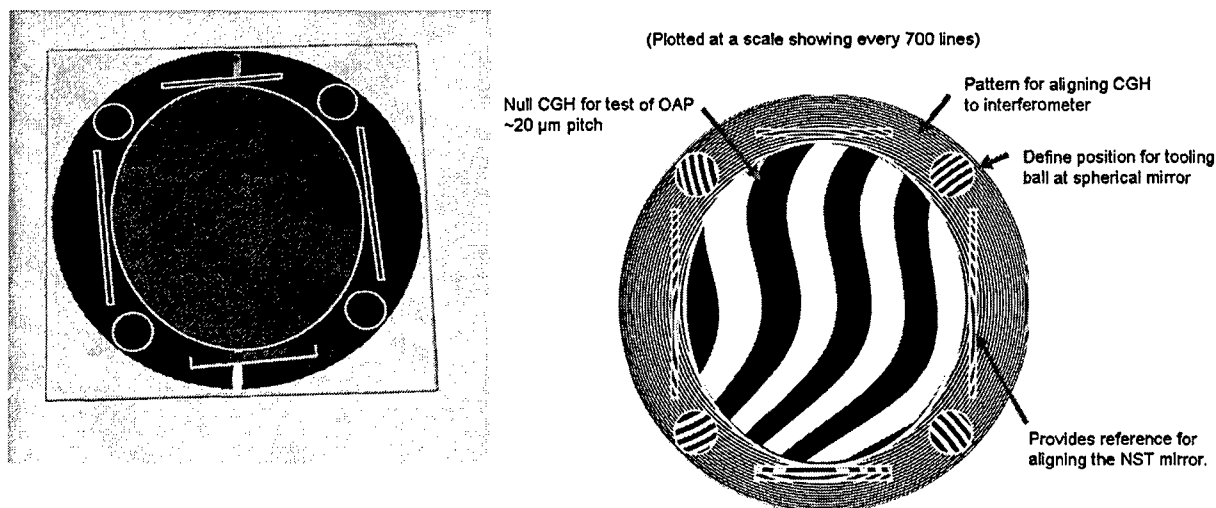
Figure 16. The CGH for the 1.7 m segment includes multiple patterns for alignment as well as wavefront correction. We show the layout of the different patterns as well as a photograph of a prototype multiplexed CGH.
