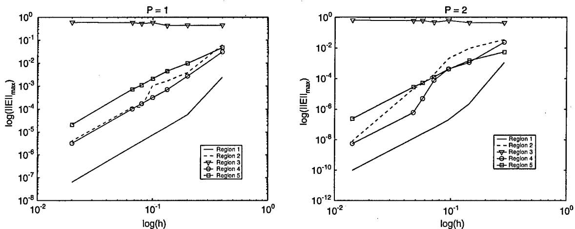
Fig. 6. Rates of convergence for problem (3.3) on meshes have 7 \times 5 , 14 \times 10 , 21 \times 15 , 28 \times 20 , 35 \times 25 , 42 \times 30 and 140 \times 100 elements on Regions 1–5 with p = 1 (left) and p = 2 (right).
