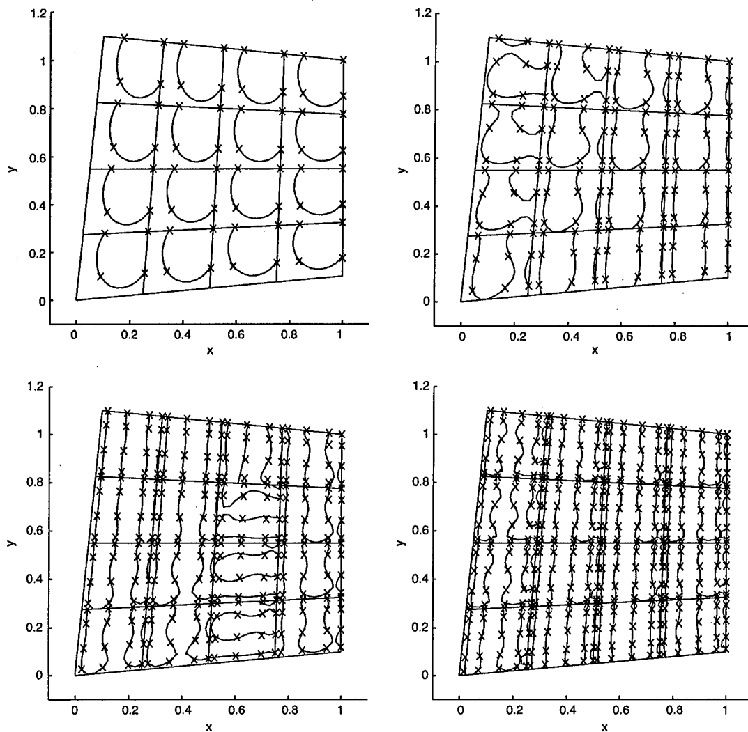
Fig. 1. Zero-level curves of the error for Example 1 using p = 1, 2, 3, 4 (upper left to lower right). Radau points are shown with an 'x'.
