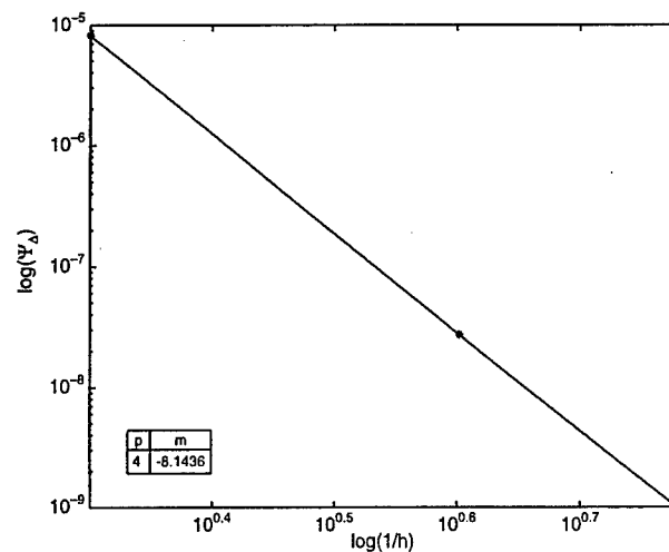
Fig. 3. The error in the flux \Psi_d on the outflow boundary of the first element versus 1/h in the log-log scale for Example 2.
