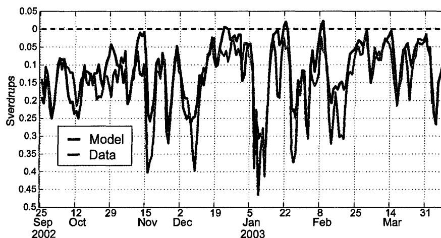
Figure 6. The western Adriatic current causes southward water transport along the Italian coast. Model results (blue) match the timing and often the magnitude of transport estimated from an array of four acoustic Doppler current profiles on a transect near Senigallia (see Figure 5b).
