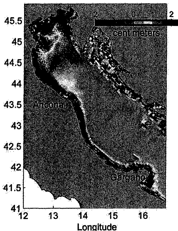
Figure 7. (a) Results of sediment-transport simulations for nine months (November 2002 – May 2003) reveal patterns of deposition for (a) fast-settling aggregates (1 mm/s) and (b) slow-settling particles (0.1 mm/s) supplied by rivers. The depositional patterns are dominated by local deposition of material from the Po River in the northern Adriatic and by southward dispersal of Apennine sediment along much of the Italian coast. Deposition is enhanced north of Ancona and the Gargano promontory, similar to the pattern seen in the Holocene thicknesses.
