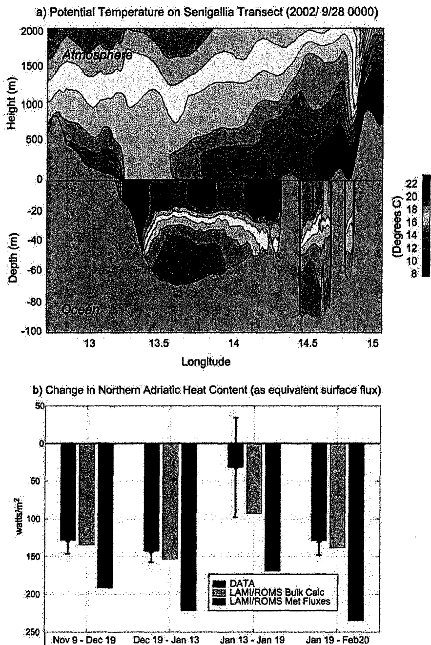
Figure 3. (a) As cold Bora winds cross the Adriatic, they flow over surface waters that are ~10 degrees warmer. This induces vigorous air-sea exchange as the atmosphere extracts heat from the ocean. The vertical contour plot shows COAMPS/NCOM two-way coupled potential temperature at the beginning of a Bora. (b) Bulk heat transfer rates calculated by ROMS fall within error bounds around fluxes estimated from satellite and in situ temperature data, but LAMI algorithms overpredict rate of heat transfer.
