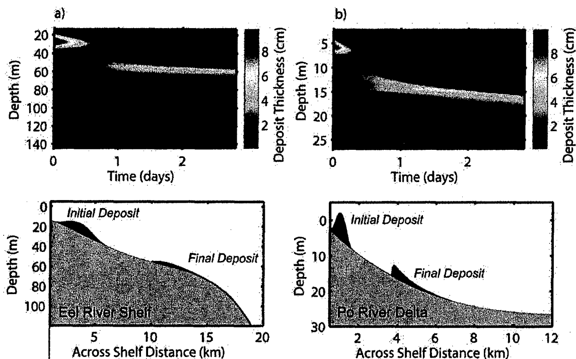
Figure 2. (a) Mud initially deposited in shallow water (20-40 m) beneath the Eel River plume is remobilized by waves and moved downslope as a gravity current, producing a final deposit in deeper water (50-60 m), according to these model simulations. The first field observations of this process were made during the STRATAFORM project, and fluid muds were again observed on the flanks of the Po River delta during EuroSTRATAFORM. The model (b) indicates that these processes occur in shallower depths in the Adriatic Sea, where waves are smaller. Note the deposits are plotted with \sim 10\times vertical exaggeration. Nittrouer et al. (this issue) show maps of the final location and thickness of fluid mud deposits after the Po flood of 2000 predicted from a two-dimensional model.
