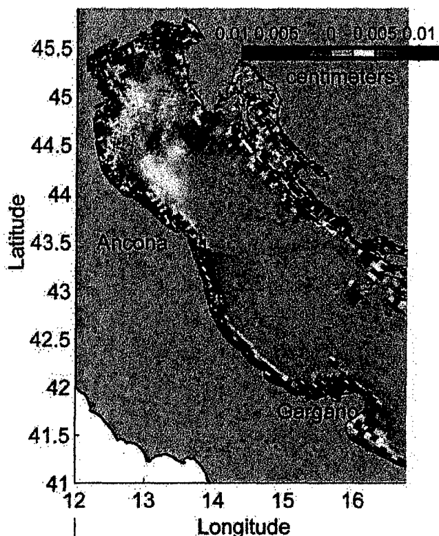
Figure 7. (a) Results of sediment-transport simulations for nine months (November 2002 – May 2003) reveal patterns of deposition for (a) fast-settling aggregates (1 mm/s) and (b) slow-settling particles (0.1 mm/s) supplied by rivers. The depositional patterns are dominated by local deposition of material from the Po River in the northern Adriatic and by southward dispersal of Apennine sediment along much of the Italian coast. Deposition is enhanced north of Ancona and the Gargano promontory, similar to the pattern seen in the Holocene thicknesses.
