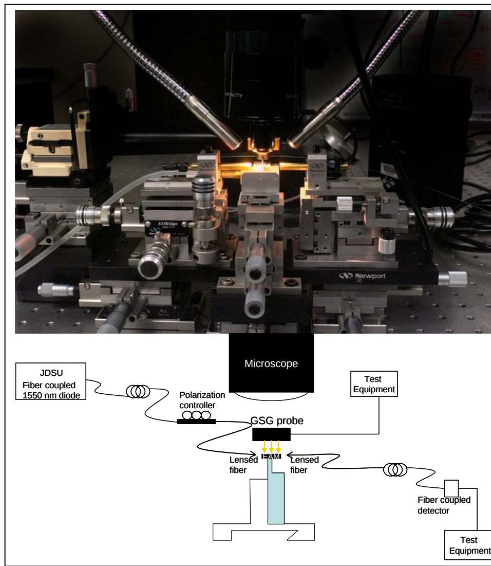
Figure 4-5. Experimental setup for testing EAMs.
