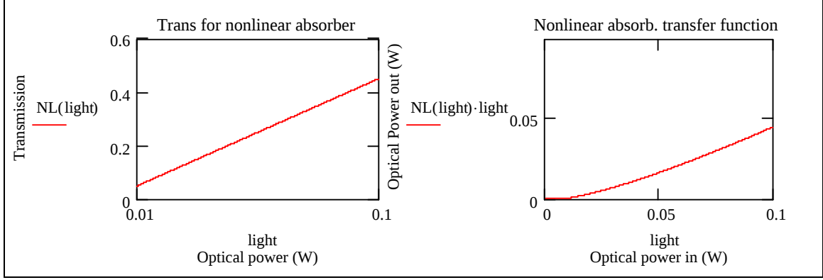
Figure 3-16. A hypothetical nonlinear absorber with a transmission that changes with optical input power. The transmission curve is a line on a semi-log graph with non-zero slope. This produces an optical transfer function that has an x \cdot \log(x) characteristic.
