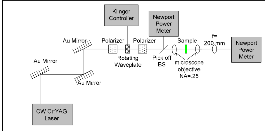
Figure 3-8. Experimental setup for nonlinear transmission measurements.
