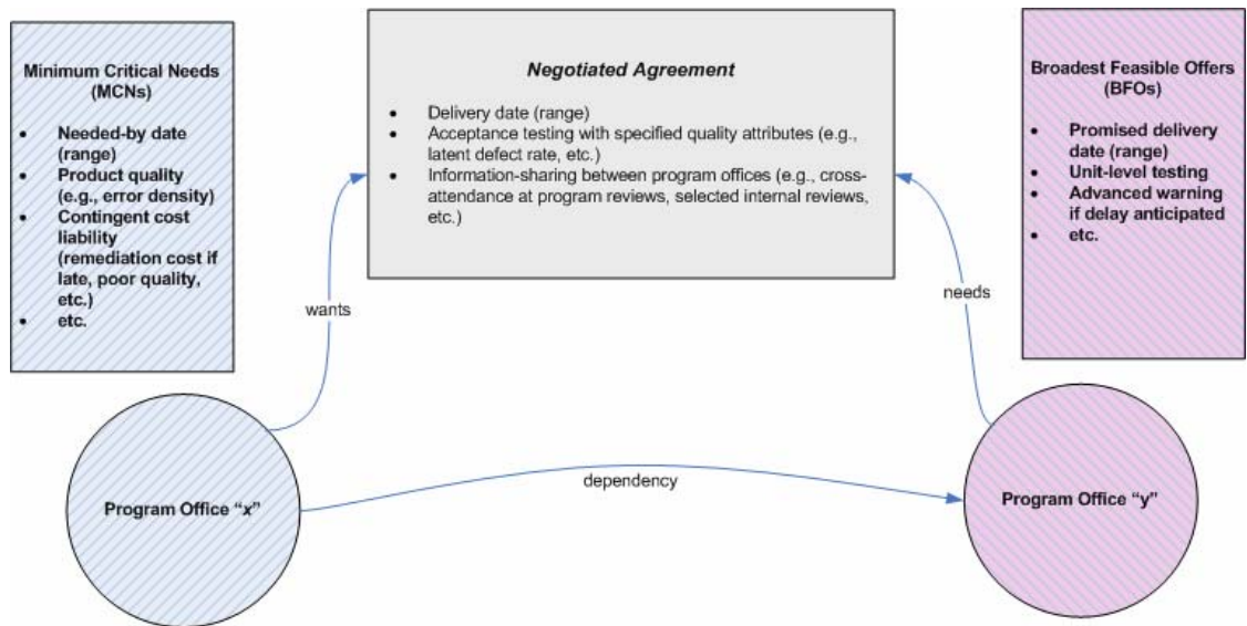
Figure 4: Arc-centric Interoperability Map
