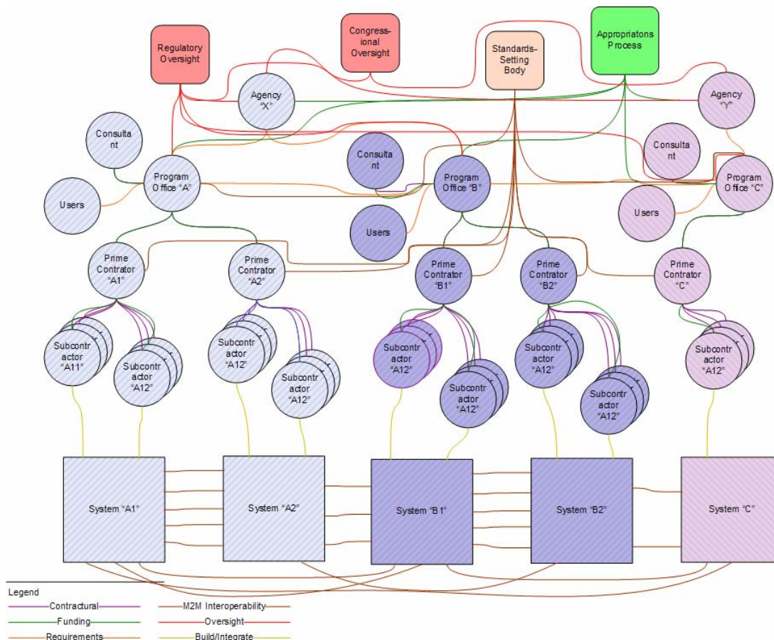
Figure 2: Context Interoperability Map
