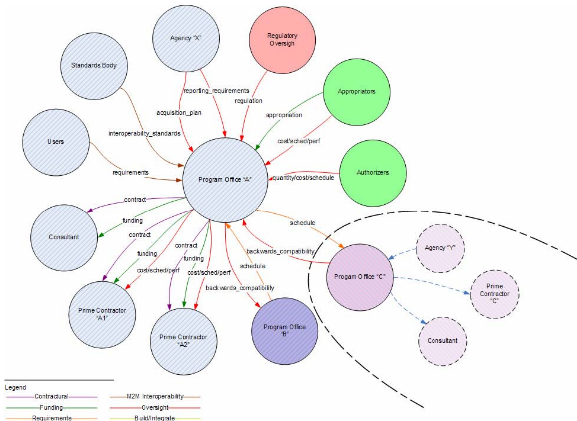
Figure 3: Node-centric Interoperability Map
