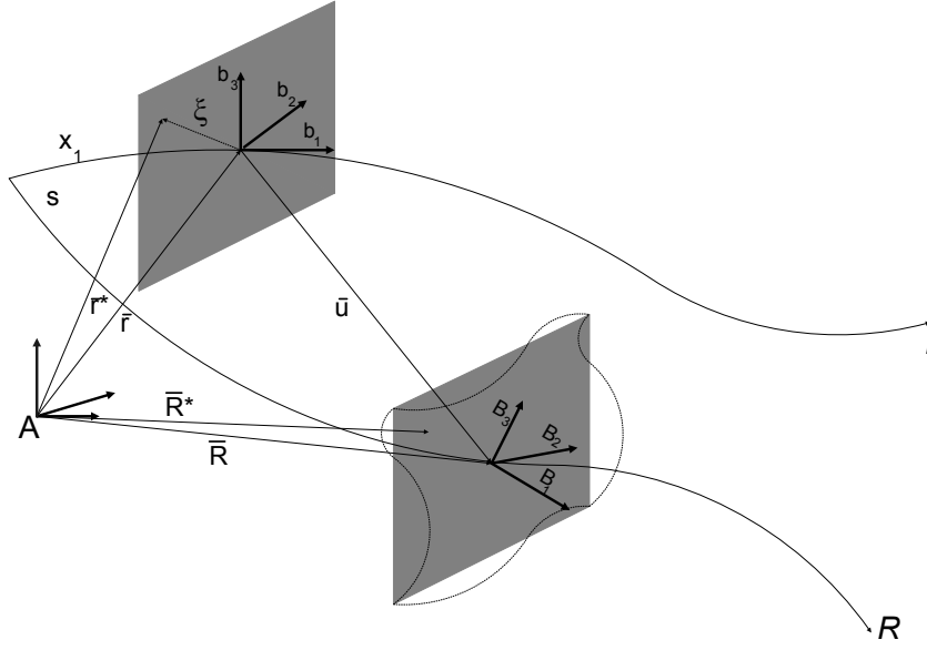
Figure 3.1: Geometry Schematic
