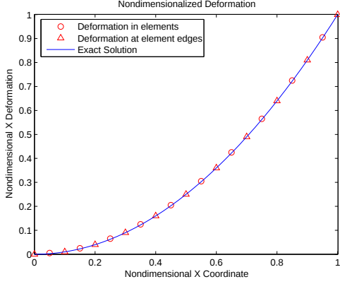
(a) Tip Moment Configuration
