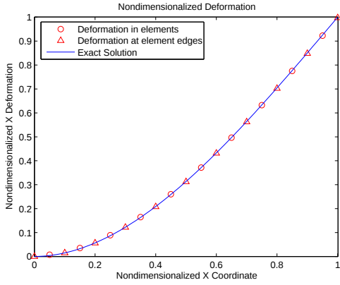
(a) Tip Load Configuration
