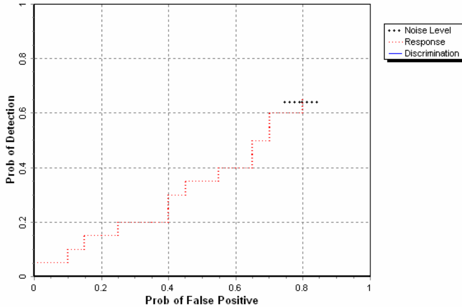
Figure 2. AMOS/towed blind grid probability of detection for response and discrimination stages versus their respective probability of false positive over all ordnance categories combined.
