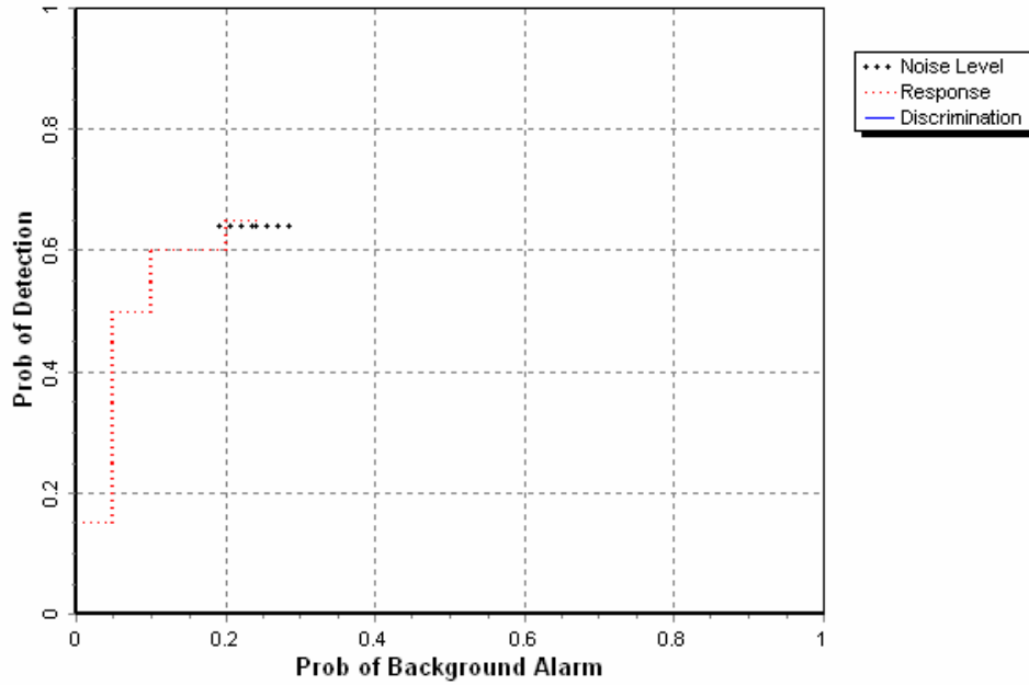
Figure 3. AMOS/towed blind grid probability of detection for response and discrimination stages versus their respective probability of background alarm over all ordnance categories combined.
