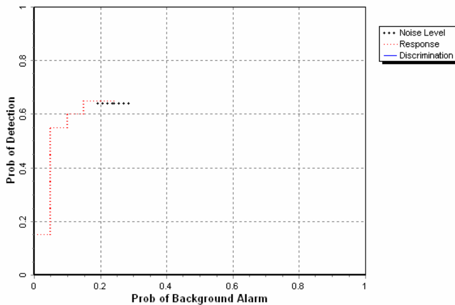
Figure 5. AMOS/towed blind grid probability of detection for response and discrimination stages versus their respective probabilities of background alarm for all ordnance larger than 20 mm.
