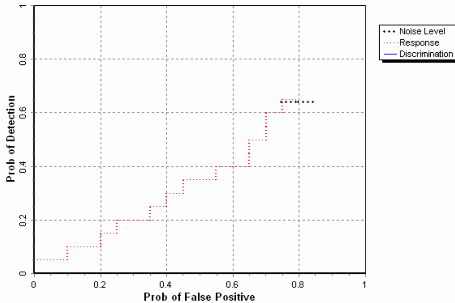
Figure 4. AMOS/towed blind grid probability of detection for response and discrimination stages versus their respective probability of false positive for all ordnance larger than 20 mm.
