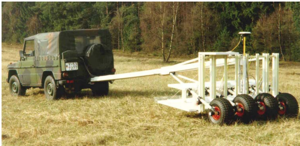
Figure 1. Demonstrator's system, vehicle based Multi Channel Detector System (AMOS).
