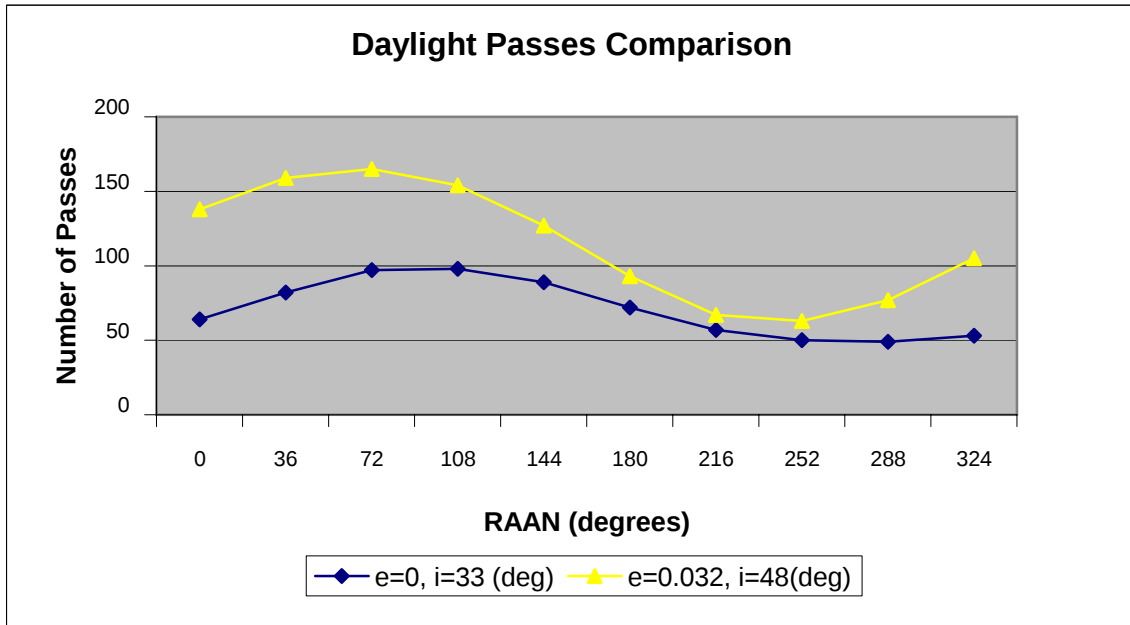
Figure 23: Daylight Passes comparison for a satellite with different eccentricity and inclination for a 30-day perion.
