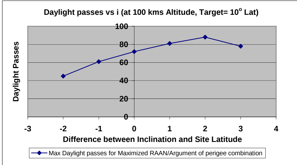
Figure 5: Daylight Passes for a satellite at 100km altitude as inclination changes with respect to target latitude. Data collected over a 30-day period for each delta i . ( \Omega , \omega are chosen to maximize daylight passes)
