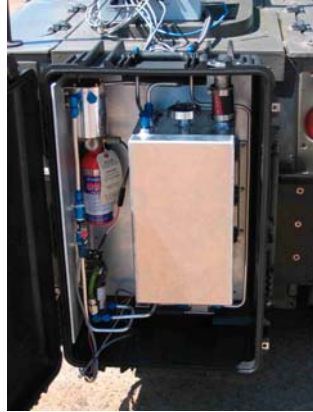
Fig. 8. AUMS Refueling Case
