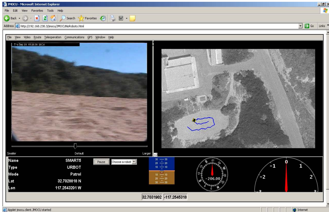
Figure 6. Web Interface Client
