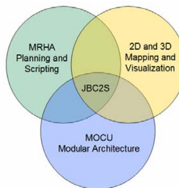
Figure 2: JBC2S architecture.
