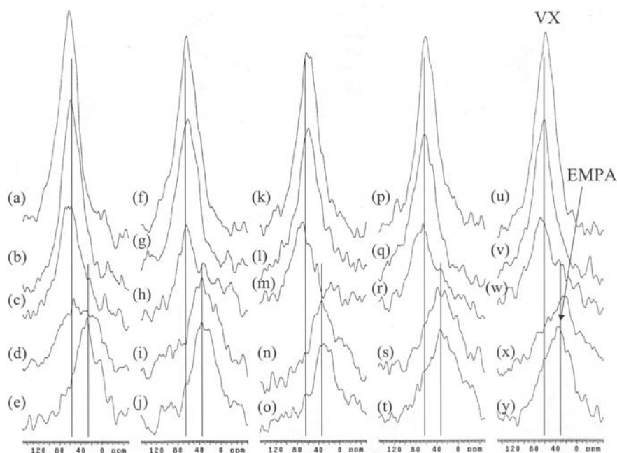
FIGURE 1. Selected ^{31}\text{P} NMR spectra obtained for VX added to concrete coupons at (top to bottom) 1 h, 5 h, 29 h, 4 days and 11 days: one-4 \mu\text{L} drop (a-e); two-2 \mu\text{L} drops (f-j); four-1 \mu\text{L} drops (k-o), eight-0.5 \mu\text{L} drops (p-t) and twenty-0.2 \mu\text{L} drops (u-y).
