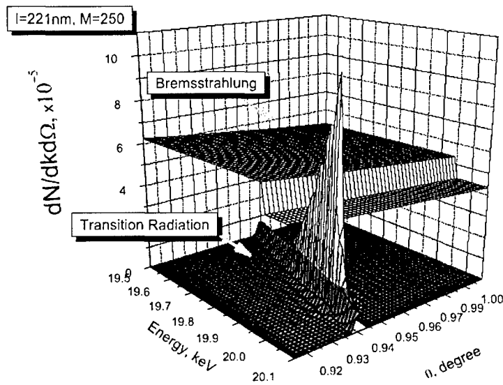
Fig. 2. The theoretical radiation spectrum of 250-period Ag/Mo nano-structure (total width \approx 55\mu\text{m} ).
