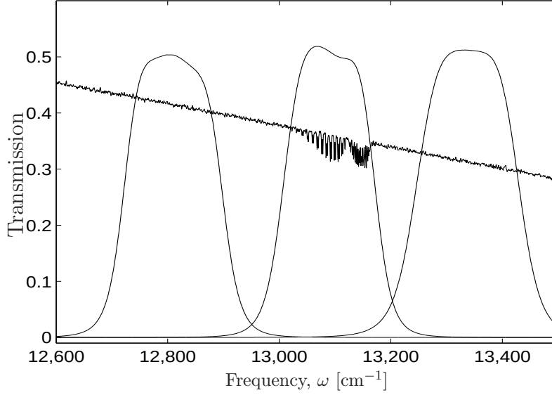
Figure 6.8: Measured spectrum (normalized to unit maximum) with filter functions overlayed. The vertical scale represents transmission, T , for the filters, or normalized intensity for the spectrum.
