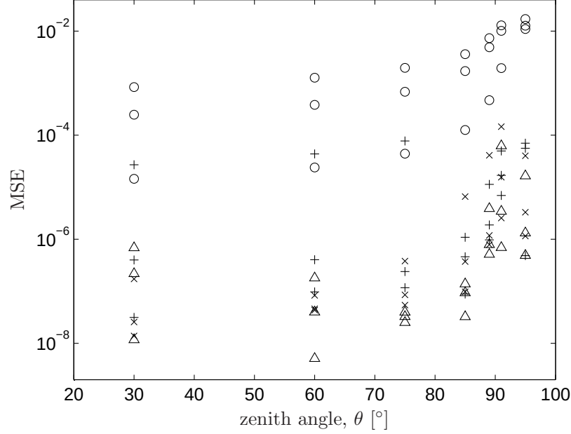
Figure 4.8: MatLab fit results for 21 different cases to compare equations. \times = equation (4.18); + = equation (4.19); \circ = equations (4.20) and (4.9); \triangle = equations (4.20) and (4.13).
