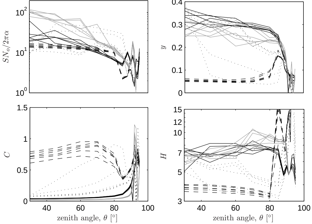
Figure 4.10: Optimized fit coefficients for eqn (4.20) (with eqn (4.13) for \Lambda ). As in Figure 4.9, line styles indicate sensor altitude: (--) = 5 km; (...) = 10 km; (-.) = 15 km; (-) = 20 km. The behavior of these curves suggests the optimization may be under-constrained.
