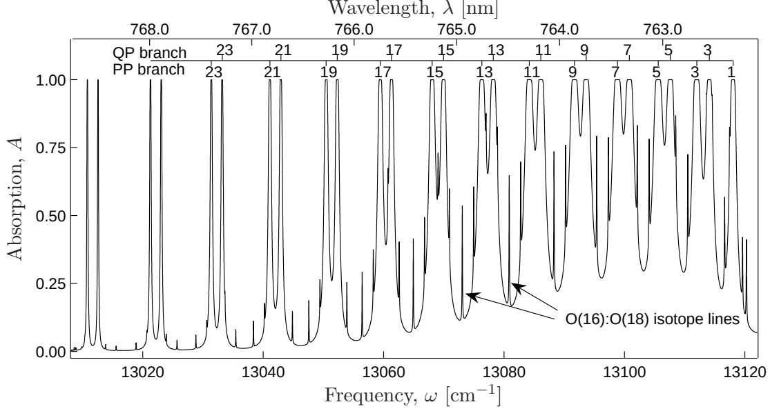
Figure 2.3: Modelled high-resolution absorption spectrum (calculated by FASCODE for 25km horizontal path with sensor located 5km above sea-level) showing the QP and PP branches. The line labels represent the rotational quantum number of the absorbing molecule, J'' . The finer, unlabelled lines are absorption by the less abundant isotope [2].
