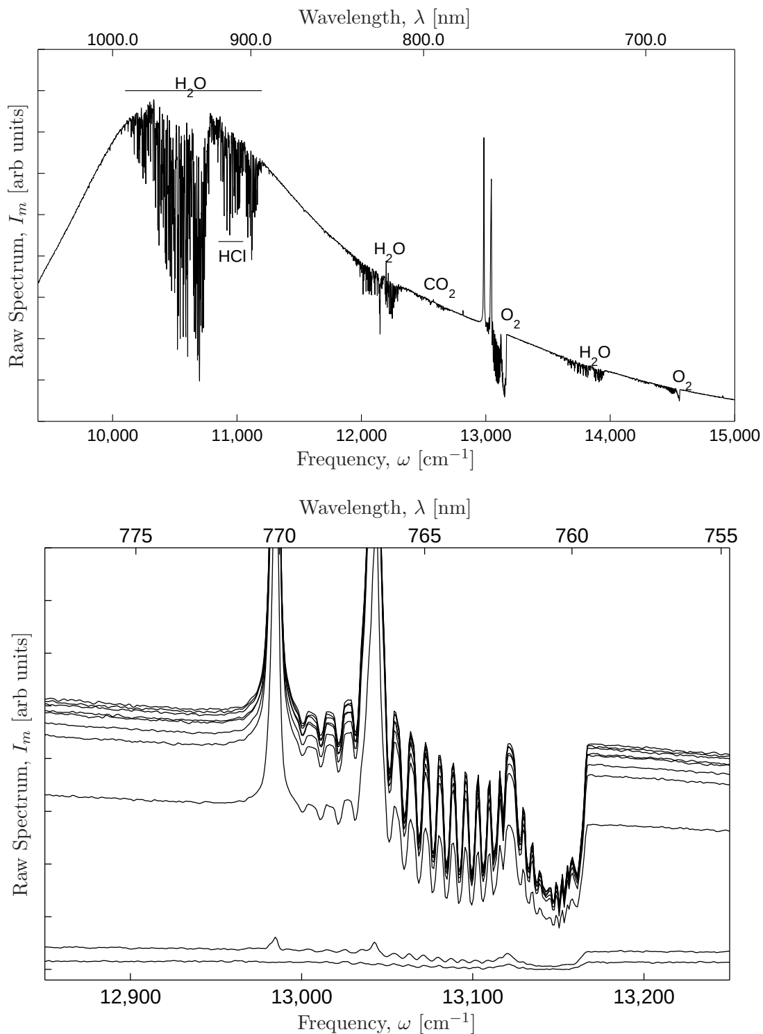
Figure 3.9: Top: single raw spectrum from SRM test, with major absorption bands identified. Bottom: the \text{O}_2(0 \rightarrow 0) band region for all ten measurements, showing the large potassium emission doublet.
