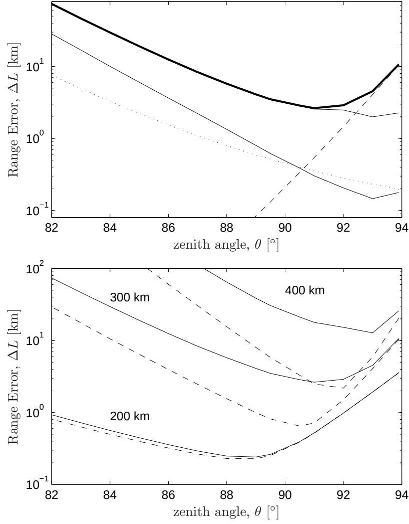
Figure 6.7: Range Errors for ABL scenario.
