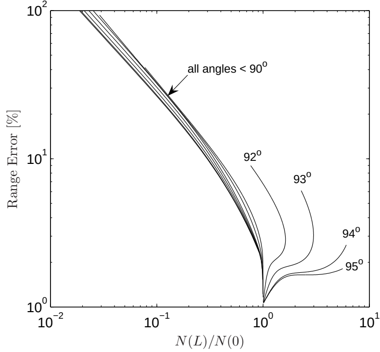
Figure 6.3: Range Error (in %) assuming s_A/\bar{A} = 1\% . All up-looking cases are very tightly grouped on this plot regardless of sensor altitude or zenith angle. Down-looking cases are more complex; curves shown are for altitude of 15 km.
