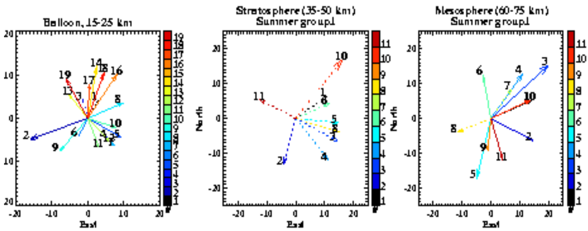
Figure 4. Distributions of propagation direction and horizontal phase speed for gravity waves inferred from a hodograph analysis of balloon and falling sphere data during the summer MaCWAVE salvoes. The trend is toward an increasing eastward propagation bias with increasing altitude, consistent with expectations of filtering theory.
