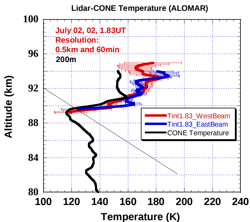
Figure 3. Temperature profiles obtained with the Weber lidar in the east (blue) and west (red) beams and with the CONE ionization gauge aboard the MIDAS rocket during the first summer MaCWAVER/MIDAS salvo. Differences between the profiles are due to different locations in a very dynamically active mesopause gravity wave field. Spacing
