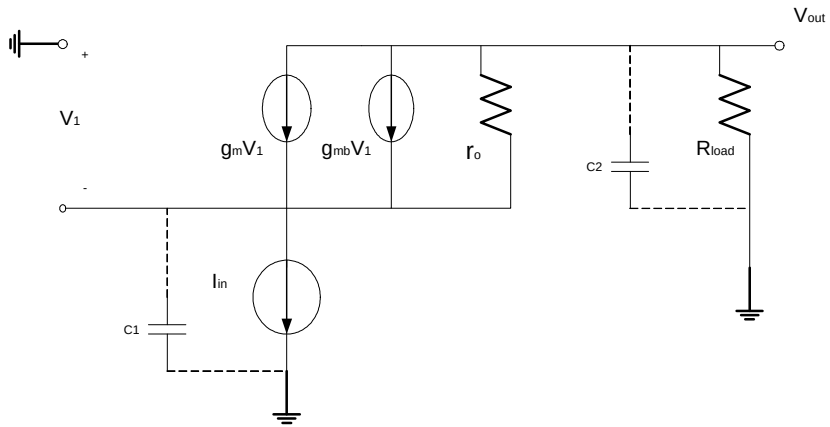
Figure 18. Small signal model of TIA
