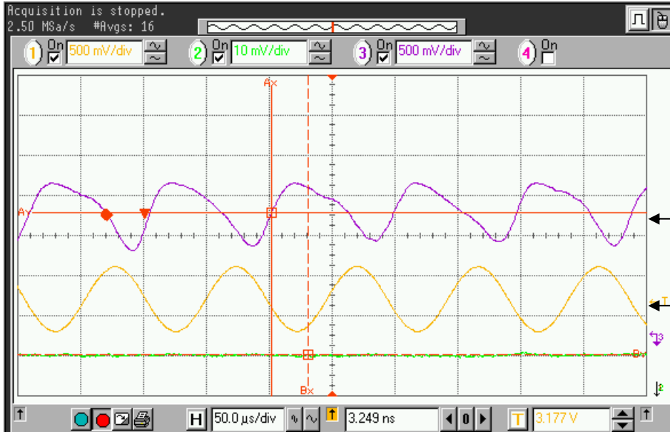
Figure 35. TIA testing waveforms. (From Agilent Infinium oscilloscope)
