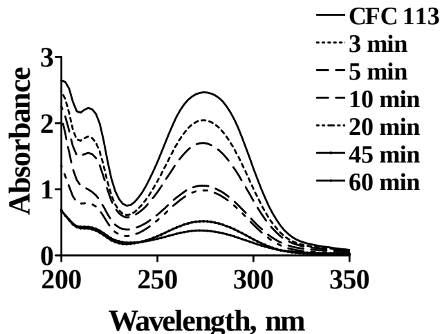
Fig. 3. UV spectra during oxidation of 0.4 \mu moles of paraoxon with 3 \mu moles of gaseous DMDO. Exposure to CFC 113 for 60 minutes is the negative control.
