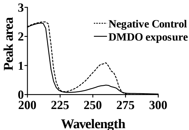
Fig. 2. UV spectra of the reaction between 96 \mu moles of DPCP and 54 \mu moles of gaseous DMDO. The negative control was CFC 113.
