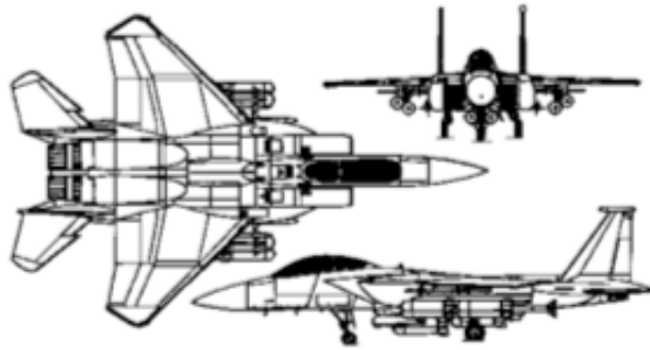
Figure 6. F-15E Line Drawing
