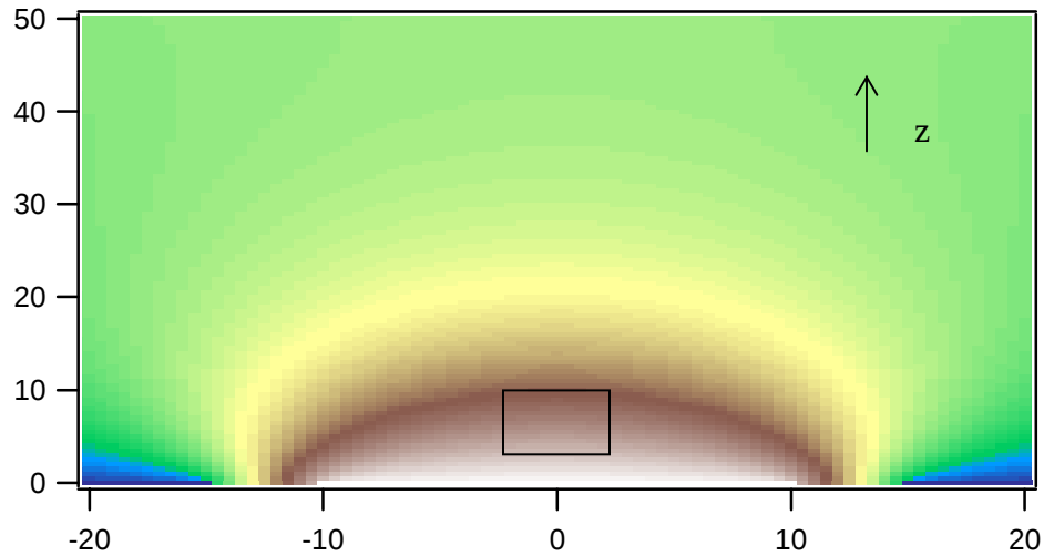
Figure 35. The image of a potential field inside KTP with an electrode configuration as described in Figure 34(cathode is white and anodes in blue). The typical waveguide dimensions are 4 \mu\text{m} wide and 8 \mu\text{m} deep (axes are in \mu\text{m} ).
