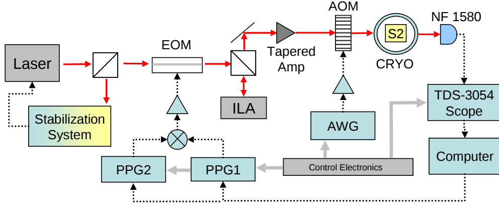
Figure 16. Experimental set-up for DSB PAWG. EOM is the electro-optic phase modulator, which is driven by two pulse pattern generators (PPG). An injection locked amplifier (ILA) is use to boost the output of the EOM to a level acceptable for the tapered amplifier. The acousto-optic modulator (AOM) driven by a low bandwidth arbitrary waveform generator (AWG) creates the multiple sidebands. The cryostat (CRYO) holds the S2 material at 4K. A New Focus detector (NF1580) is used to detect the generated waveforms and capture them on a Tektronix TDS-3054 oscilloscope.
