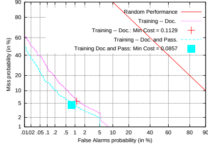
(c) TDT4 DET Plot at n = 0
