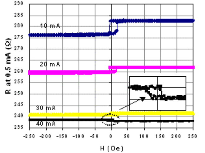
Fig. 3. Deterioration of an MTJ during writing in an improperly designed magneto-thermal MRAM element. The resistance of the MTJ is measured at 0.5 mA, after each attempted heating cycle. The inset shows the magnetization was finally reversed at 40 mA of heating current, at much higher current than the barrier could handle.
