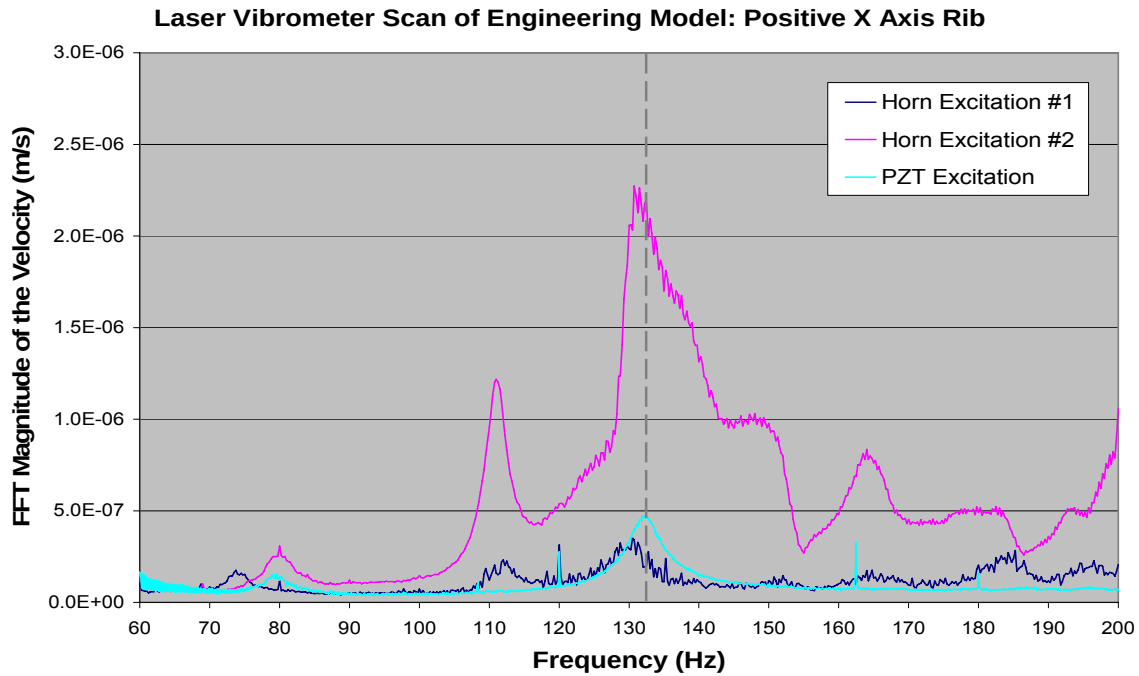
Figure 5.12 Engineering Model X Axis Laser Vibrometer Scan Results
