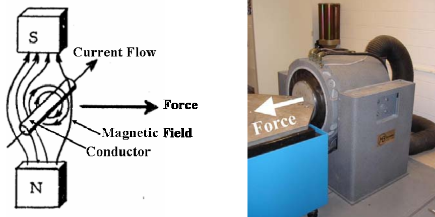
Figure 4.1 Fleming’s Left Hand Rule Utilized in an Electrodynamic Vibe Table
