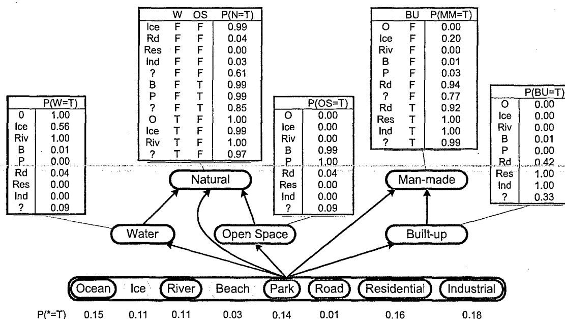
Fig. 6. Example Bayesian network illustrating the resultant structure and conditional probability tables (CPTs) that parameterize the network.
