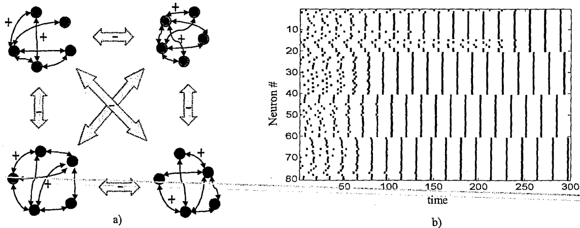
Figure 2. Connectivity pattern leading to multiple out-of-phase synchronized sub-groups. a) Schematic diagram of connectivity. Each sub-group represents 20 fully-connected neurons with excitatory connections (no delay). Each neuron has an inhibitory connection (no delay) to every other neuron that is not in its sub-group. b) Activity of neurons across time. Neurons begin with random phase, then as time progresses each sub-group becomes phase-locked within itself, and out-of-phase with every other sub-group.
