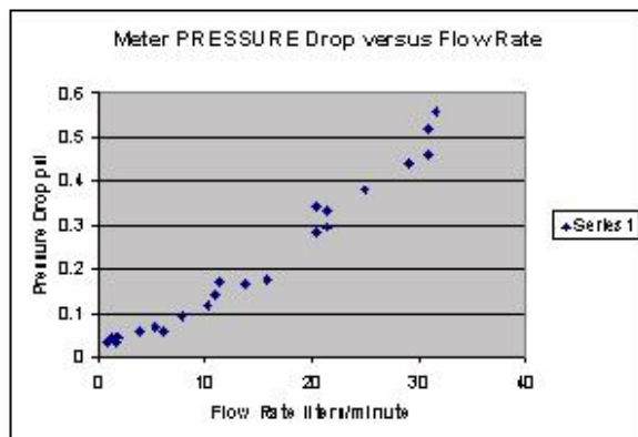
Figure 4. DryCal DC-Lite model H - Pressure drop versus flow rate.
