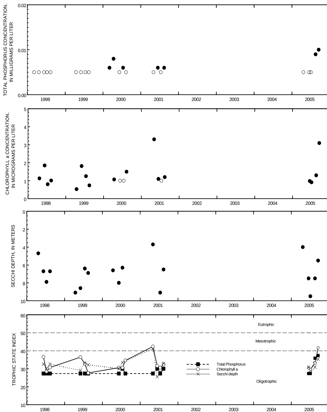
Surface total phosphorus, chlorophyll a concentrations, Secchi depths, and TSI data for Whitefish Lake, South Site near Gordon, Wisconsin.
