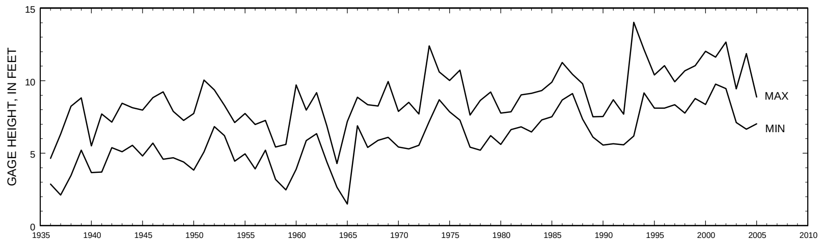
Annual minimum and maximum water levels for Devils Lake, 1936-2005.
