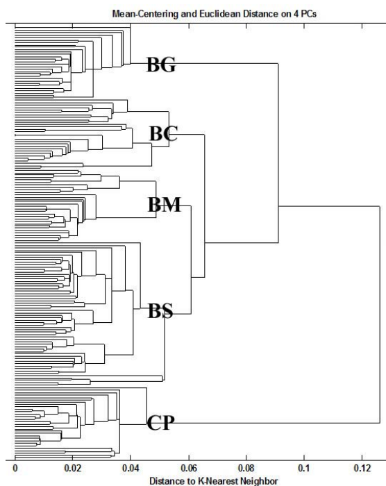
Figure 5. HCA dendrogram of autoclaved (Set 1) endospores of B. cereus (BC), B. globigii (BG), B. megaterium (BM), B. subtilis (BS), and C. perfringens (CP) illustrating clustering of species.
