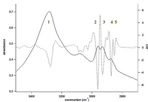
Figure 3. Absorbance (—) and 2 nd derivative (---) spectra of B. megaterium endospores from 2700-3500 \text{cm}^{-1} . Peak assignments are as follows: 1. N-H str. (amide A); 2. C-H str. of -\text{CH}_3 (asym.); 3. C-H str. of >\text{CH}_2 (asym.); 4. C-H str. of -\text{CH}_3 ; 5. C-H str. of -\text{CH}_2 associated with lipids and fatty acids. 20
