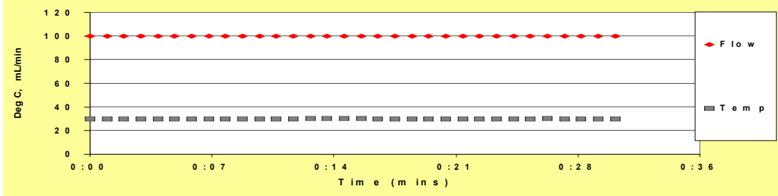
Figure 4. Wind Tunnel Temperature and Flow Control Capability as a Function of Time
