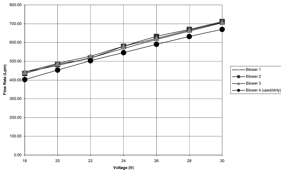
Figure 5 Brailsford motor/blower flow rate comparison.
