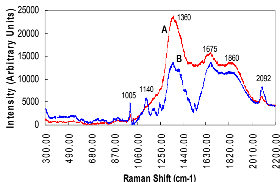
Figure 4A. Surface-Enhanced-Raman-Scattering (SERS) spectra of two different single, optically trapped Bacillus stearothermophilus (ATCC 10149) spores.
