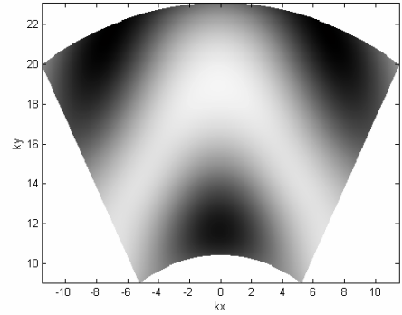
Figure 4. The radiate pattern of the calibrator in transformed domain The radiometric correction and calibration for received data in equation (5) is obtained:
