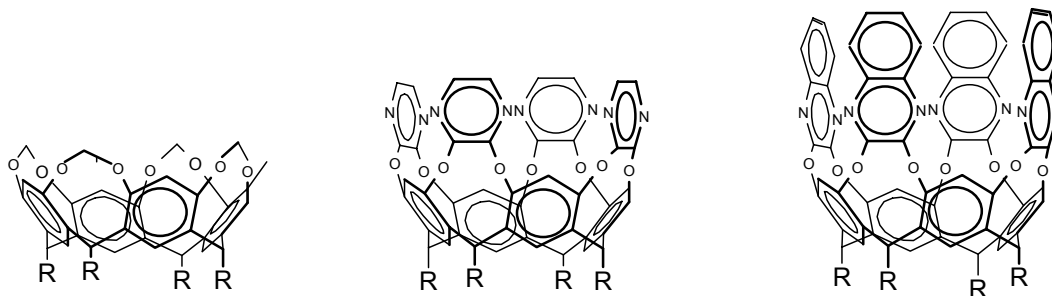
FIGURE 1. The three cavitands MeCav (methylene bridged), PzCav (pyrazine bridged), and QxCav (quinoxaline bridged) shown respectively from left to right differ both in the depth of the cavities as well as the specific interactions presented by the cavities
