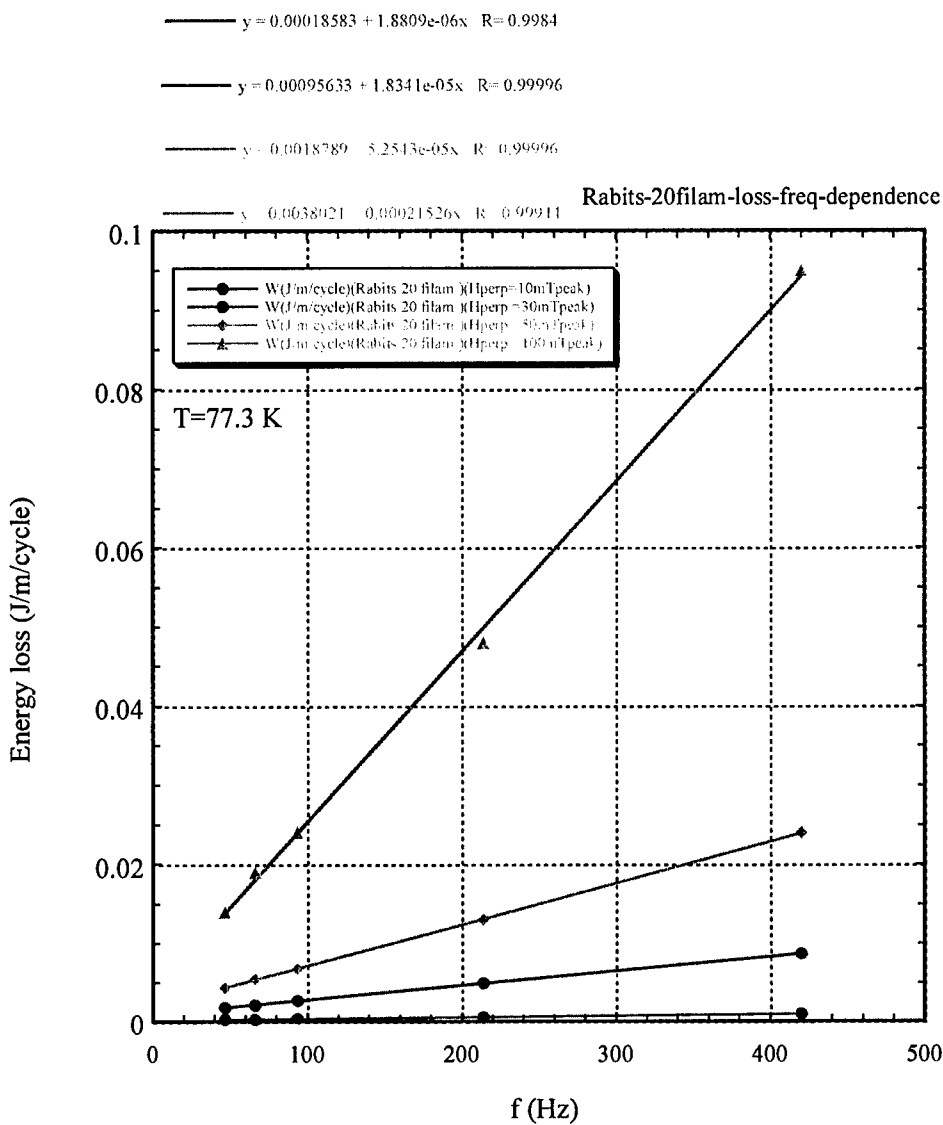
Fig. 3: Frequency dependence of the energy loss of a Rabits-20 filament sample, with no superconducting bridging between the filaments, at different magnetic fields applied perpendicularly to the broader face of the sample in a liquid nitrogen bath.
