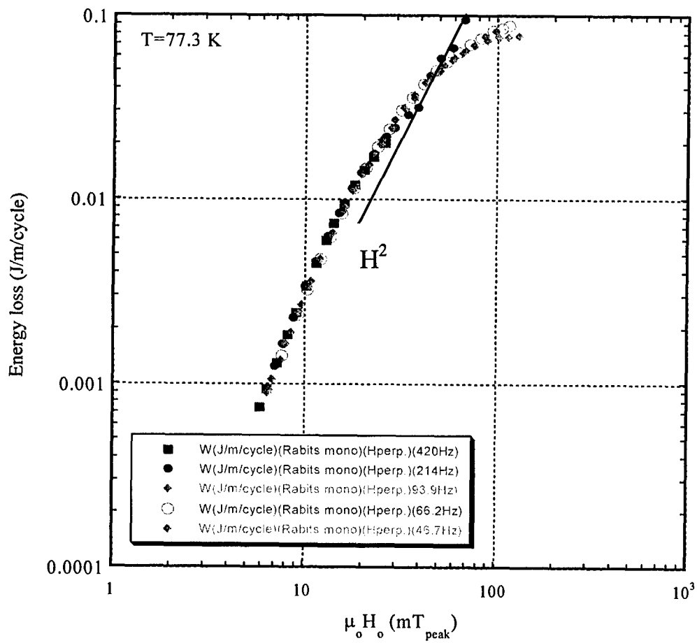
Fig. 4: Energy loss of a Rabbits-monolayer sample measured in an applied magnetic field perpendicular to the broader face of the sample at different frequencies in liquid nitrogen bath.
