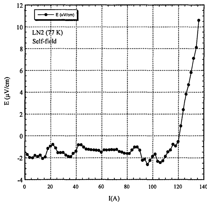
Fig. 15: DC current-voltage characteristic of Sample CM1 – filamentary part, I_c(1\mu\text{V/cm})=120\text{ A} .
