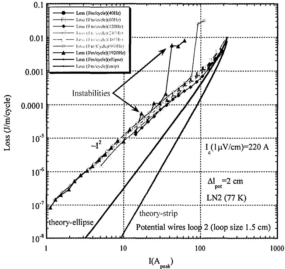
Fig. 16: Transport ac losses of Sample CM1 – monolayer part, I_c(1\mu V/cm)=220 A , measured in the frequency range 40 Hz – 2 kHz.
