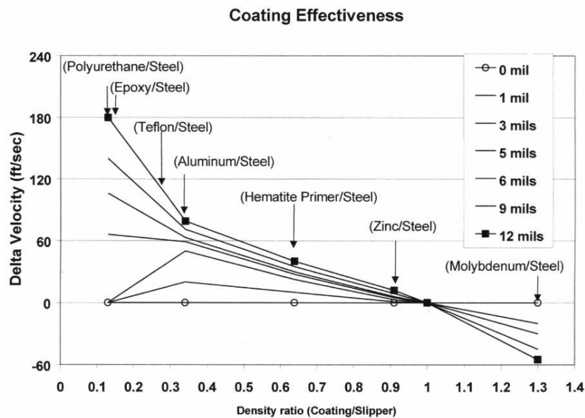
Figure 2.12: CTH Analysis of Various Coatings Effectiveness.
