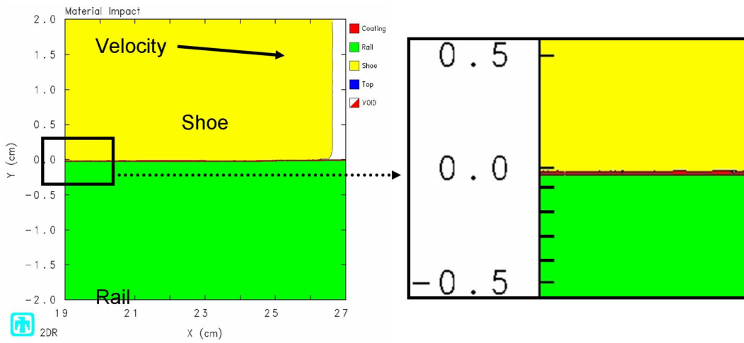
Figure 9.2: Sled, Vertical Impact of 2 m/s at 10 \mu seconds.
