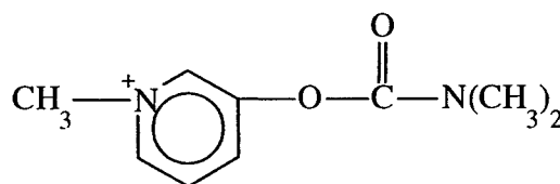
Figure 3 Structural formula of pyridostigmine.
