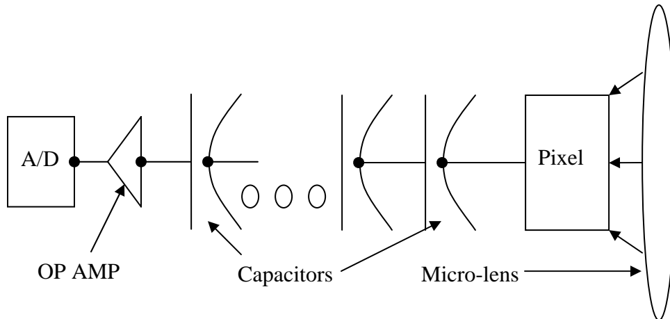
Figure 2.4 shows the circuitry connected to the pixel.
