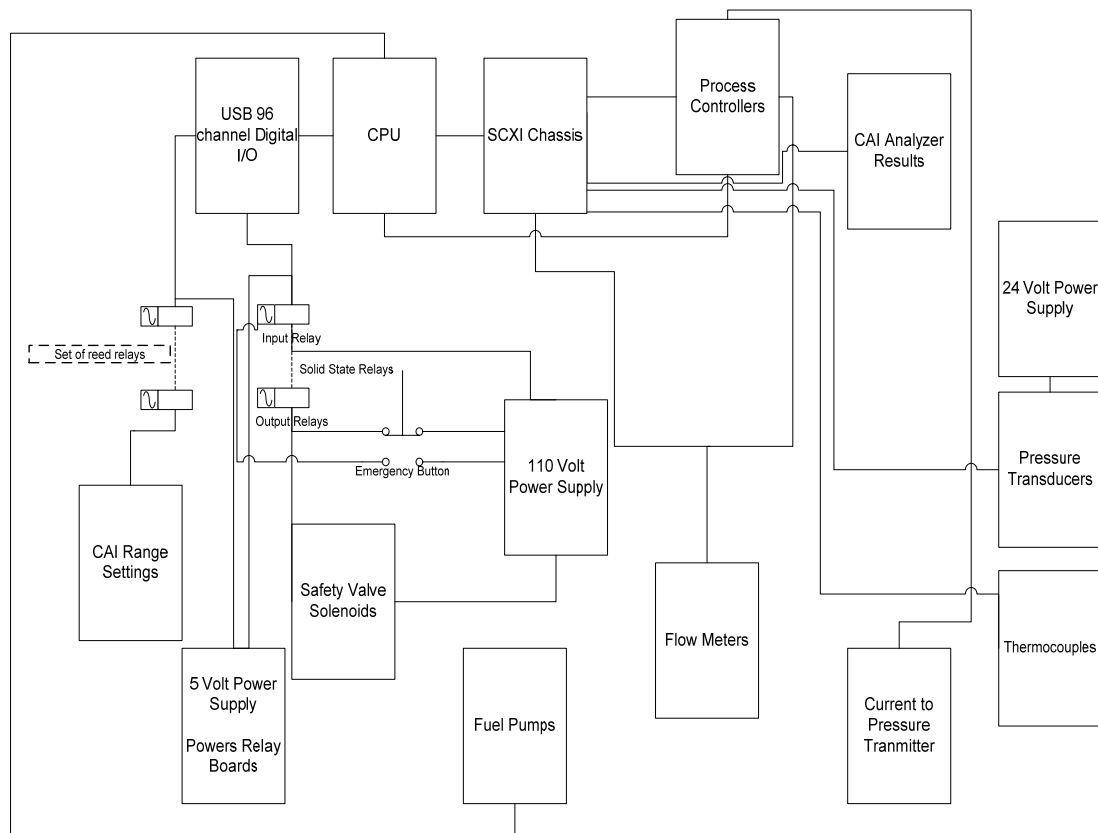
Figure 14 Wiring Diagram
