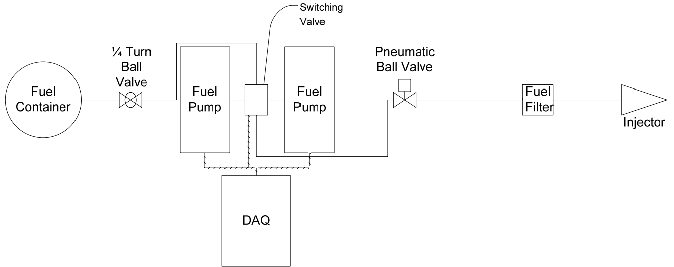
Figure 11 Fuel Line
