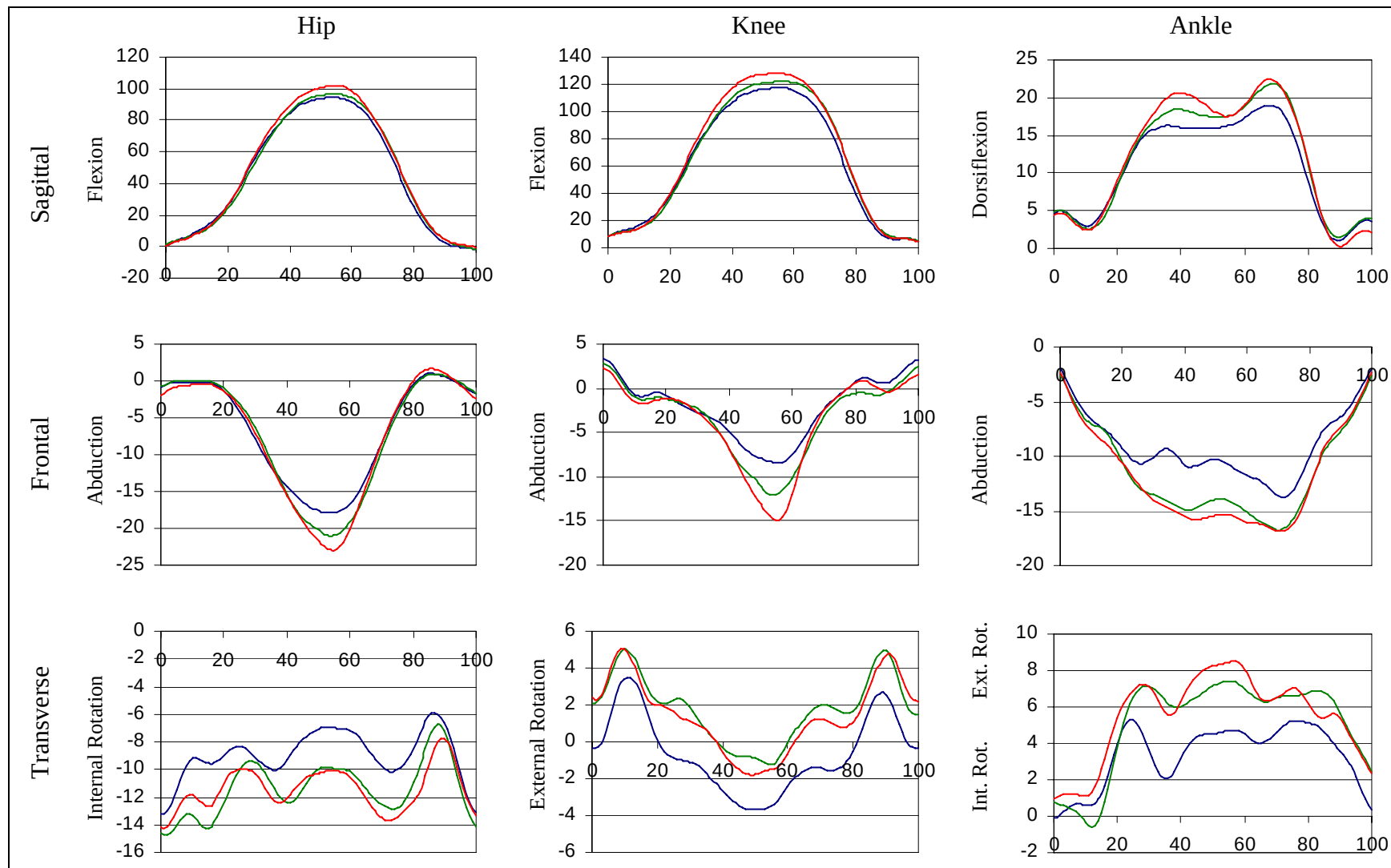
Figure D-14. Joint angles (degrees) over one cycle of left kneeling: (Blue=Baseline, Green=1-inch Sole, Red=2-inch Sole), N=12.
