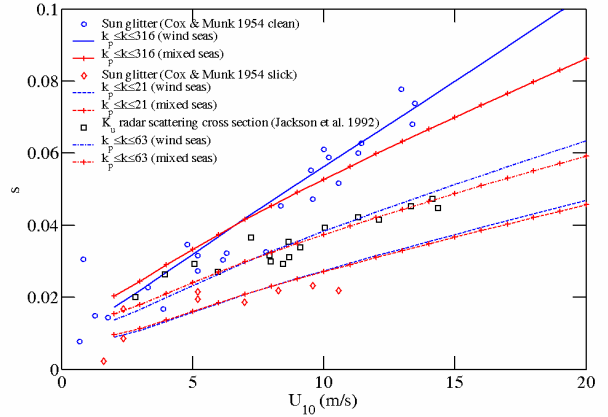
Fig. 2. Mean-square slopes integrated from k_p to different upper-bound wavenumbers, k_s . Field data from sun glitter and altimeter scattering analyses are also presented for comparison.
