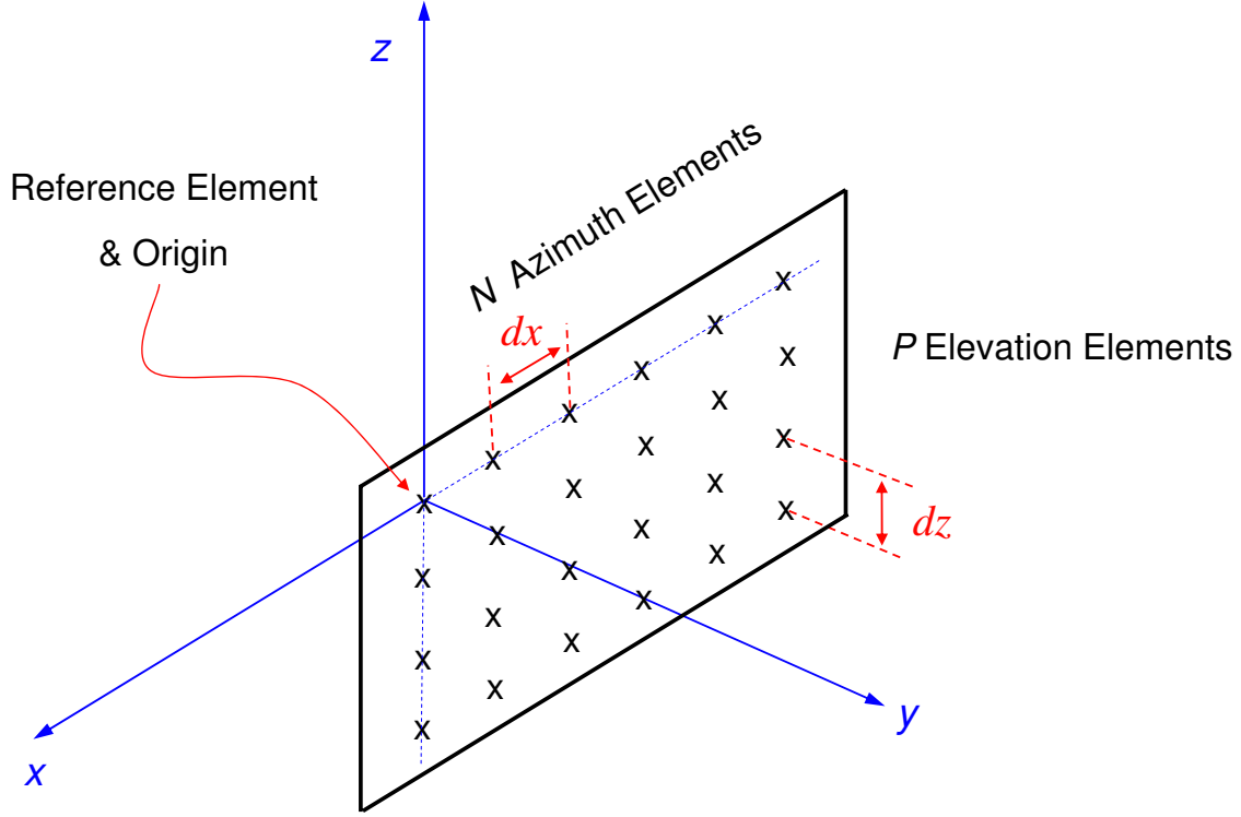
Figure 3.1: Antenna array geometry. The antenna array is oriented in the x - z plane. Its reference element, defined as the upper-left most element, serves as the origin of the cartesian and radar coordinate systems. The elements are uniformly spaced with inner-element spacings of dx in the x direction and dz in the z direction. The N azimuth channels are numbered 0 to N - 1 , and the P elevation channels 0 to P - 1 .
