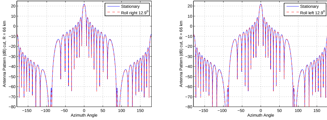
Figure 4.17: Antenna pattern azimuthal cuts at 66 km and 12.86° roll. On the left, an azimuth cut for the roll right scenario shows no difference than the roll left scenario (right). The lack of elevation definition in the linear array causes the lack of illumination difference.
