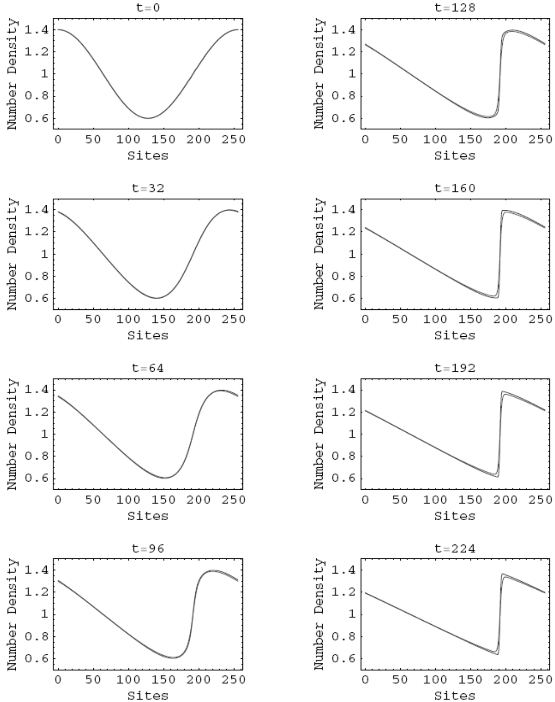
Figure 11. Numerical results of the Burgers equation simulation carried out by Yepez, along with the analytic solution. Agreement between the simulation and the analytic solution is generally very good, with slight deviations occurring at later times as a steep shock front is formed. The simulation shock front is sharper than the analytic shock. This figure was used with permission from [10].
