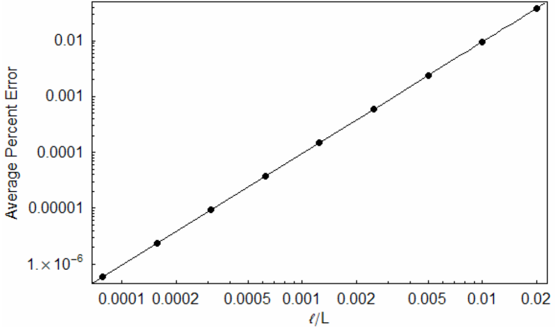
Figure 18. Log-log plot of the average percent error verses the lattice resolution. The same simulation was run with lattice lengths ranging from 50 \ell to 12800 \ell , each evaluated at 15 \tau . The slope of the best fit solid line is 2.01, indicating second order convergence in space.
