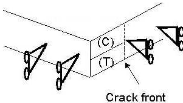
Figure 6.2 Schematic of crack insertion at the beginning of the cool-down by when the top surface is in compression, while the bottom is in tension along the x-z plane of the mesh.
