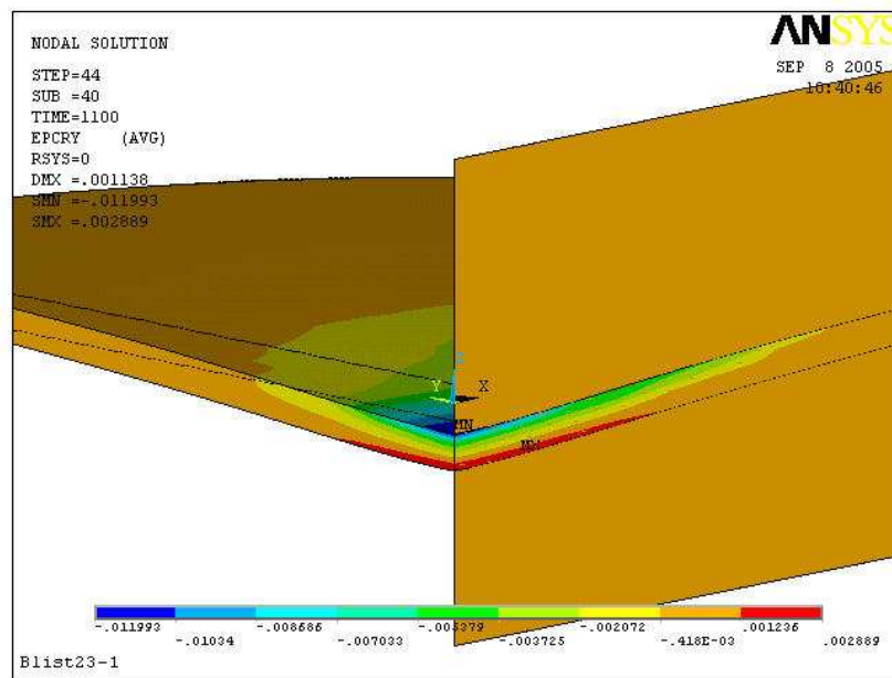
Figure 5.7 Top ANSYS plot at of the creep strain (y-direction) in the model
