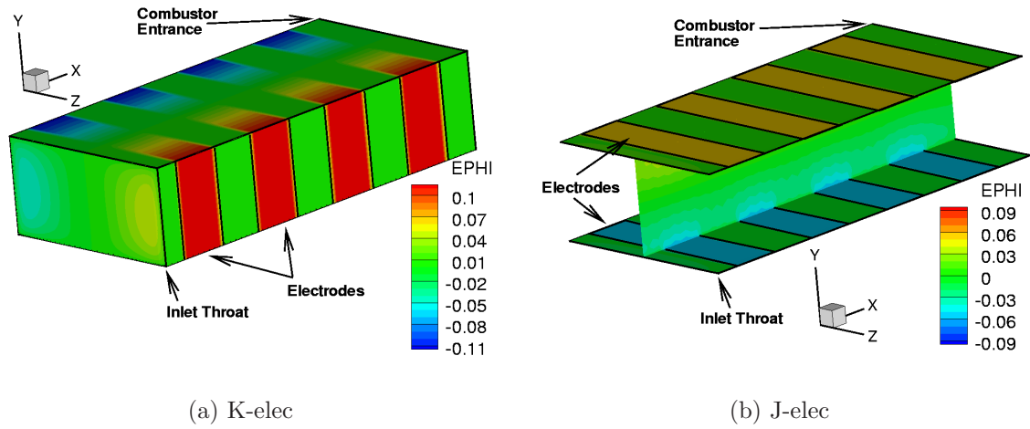
Figure 6.2: Electrode Configurations for Isolator-Based Generators with Specified Electric Potential
