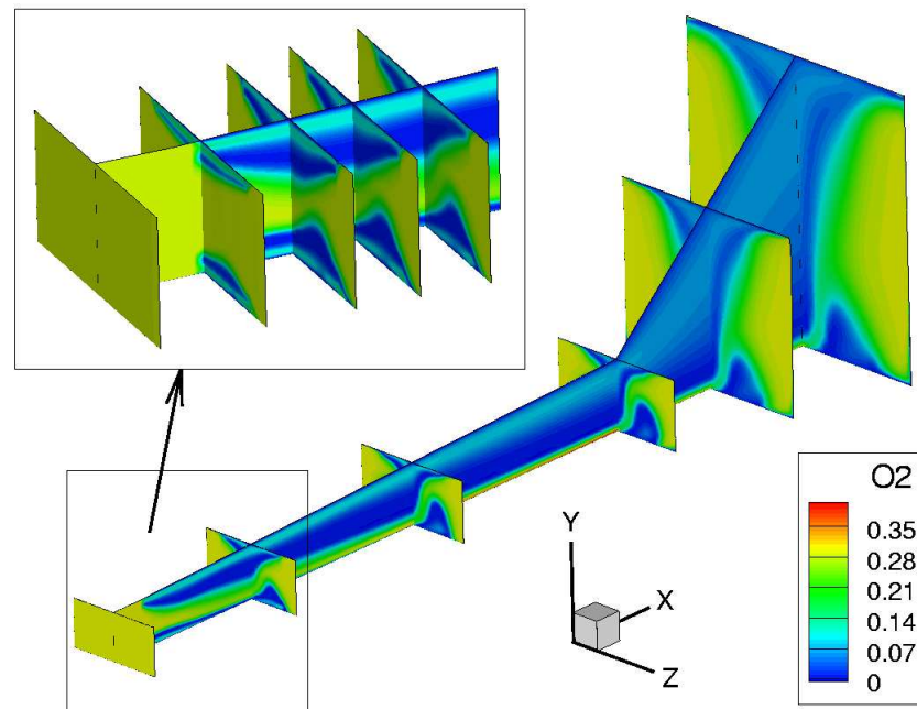
(b) Y_{O_2}
