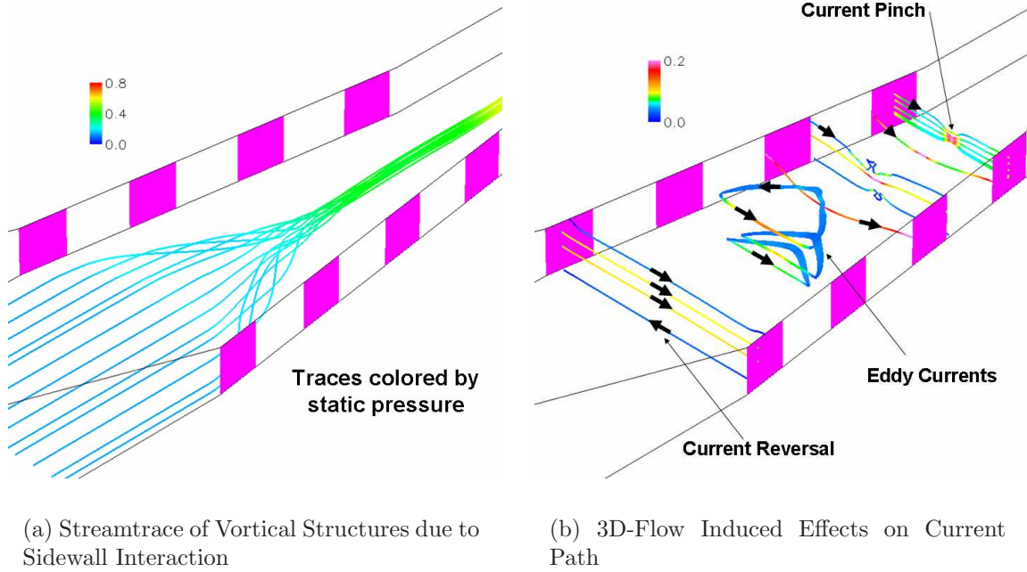
Figure 2.2: Examples of 3D MGD-Flow Interaction in AFRL Scramjet Inlet Model[21]
