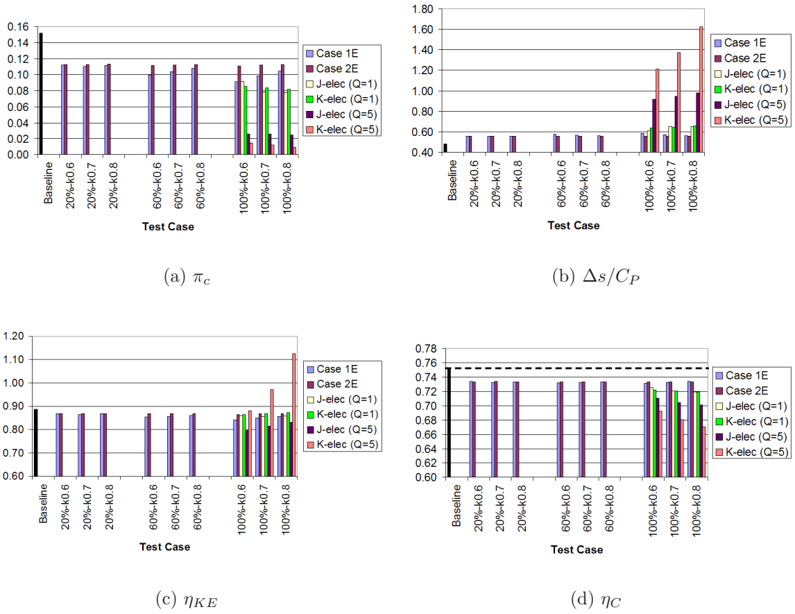
Figure 6.7: Comparison of Inlet Efficiencies for Isolator-Based MGD Power Generation
