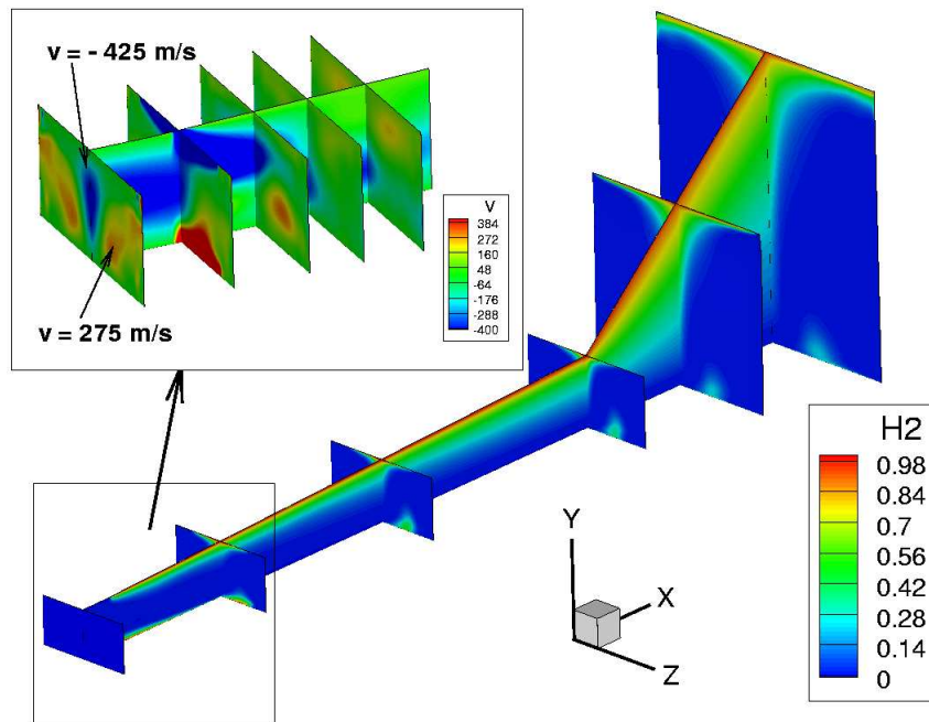
(a) Y_{H_2} with v-Velocity Contours in Inset
