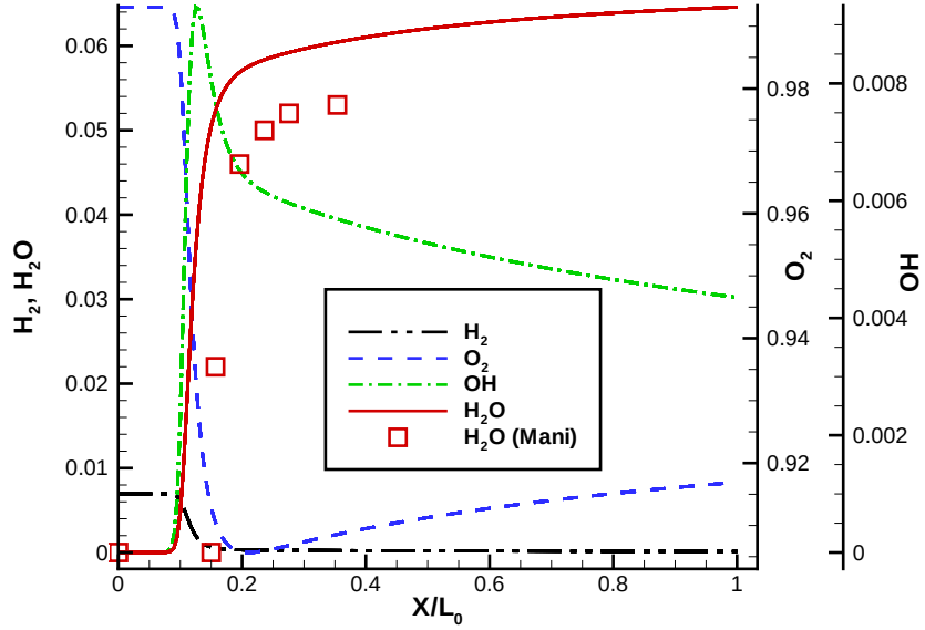
Figure 4.1: Combustion Nozzle Species Distribution
