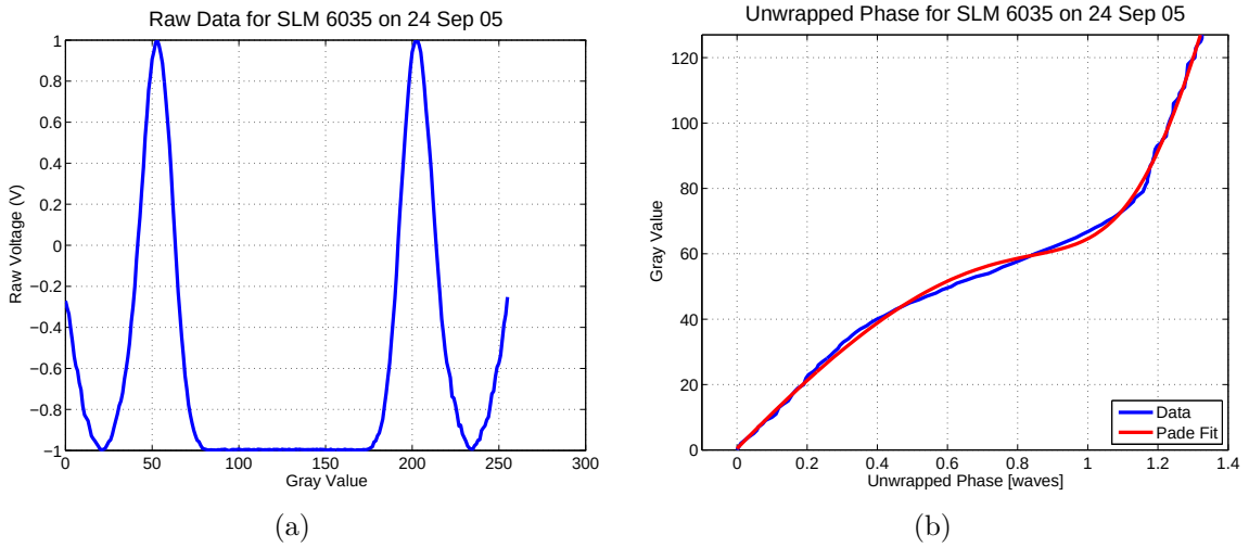
Figure 3.6: (a) Normalized raw data from the photo diode. (b) Phase to gray fit.
