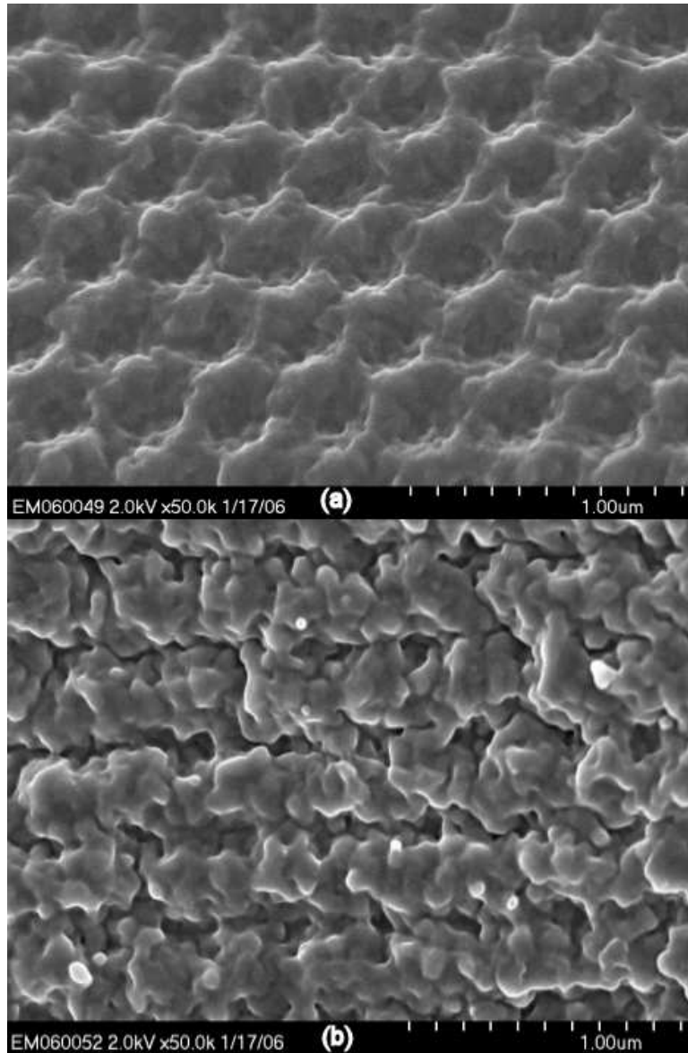
Figure 5.21: SEM of two-dimensional PhC in SU-8 fabricated by holographic lithography technique with an exposure time of (a) 9.19 seconds and (b) 9.49 seconds.
