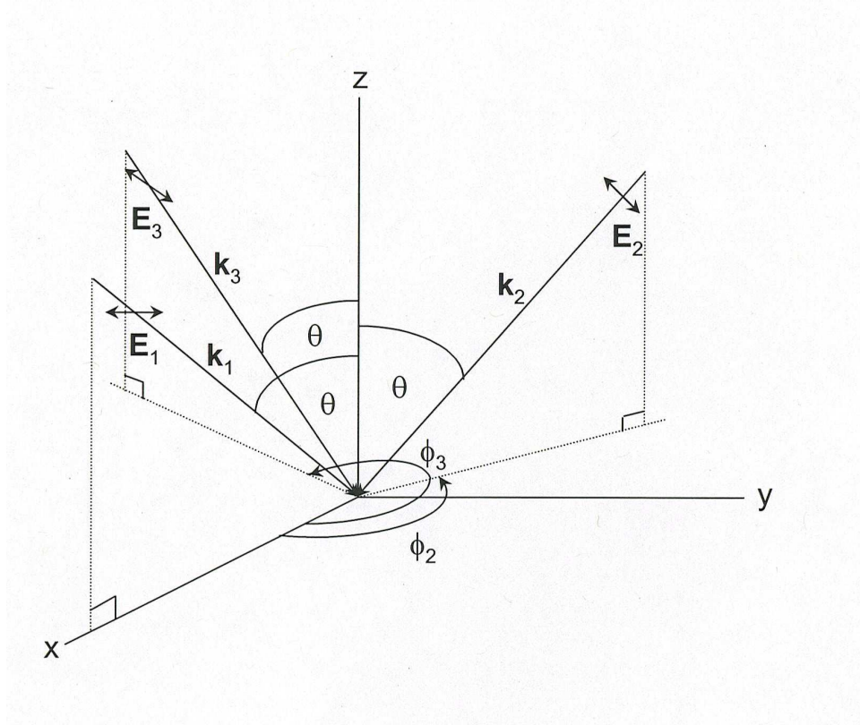
Figure E.1: The geometry that explains the equations used in the holographic polymerization/lithography process.
