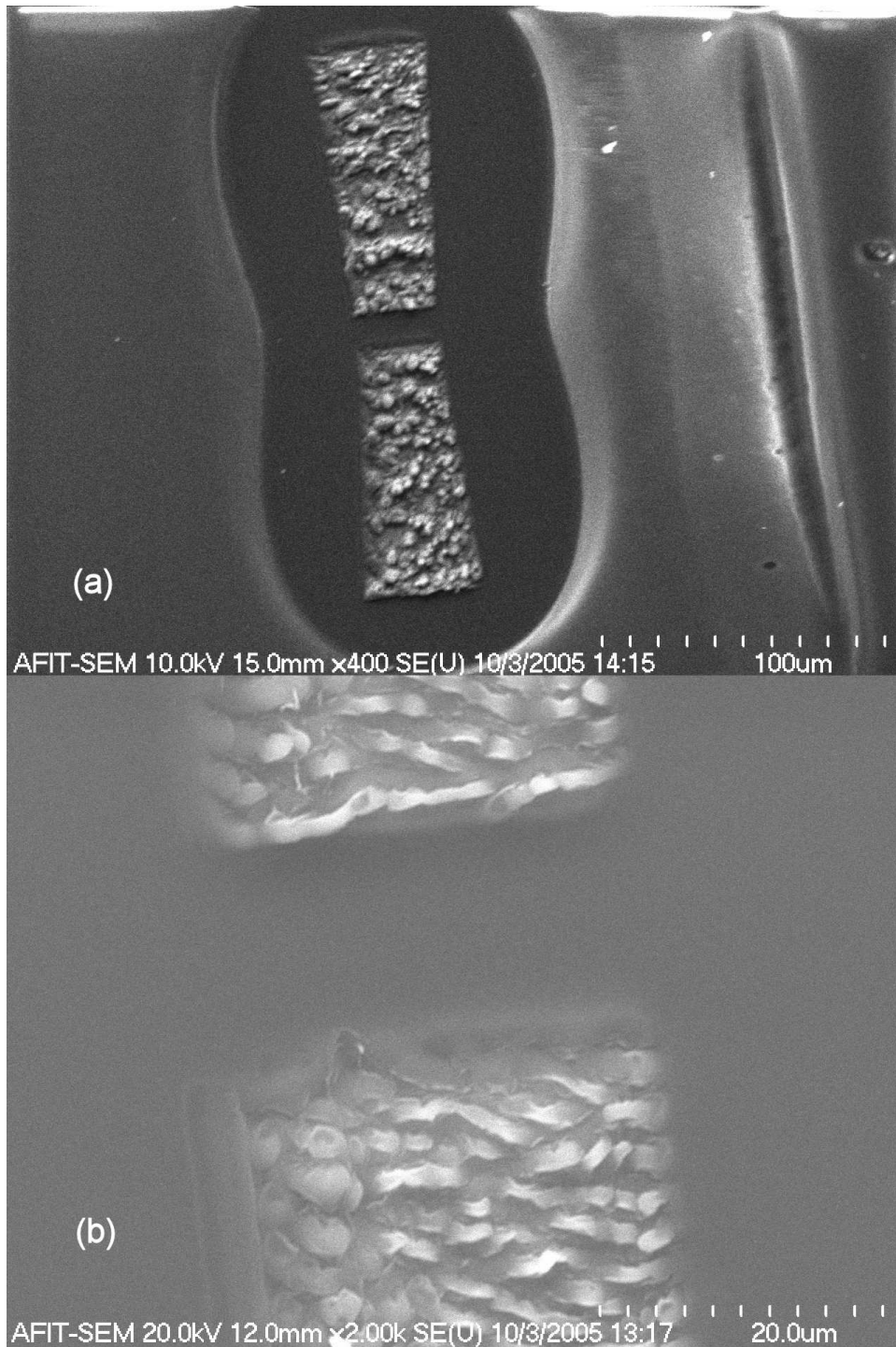
Figure 5.5: SEM image of APC channel in air, (a) with better drift correction and (b) with best drift compensation to achieve approximately 15- \mu\text{m} channel of APC in air. (b) Is also magnified to a 20- \mu\text{m} scale.
