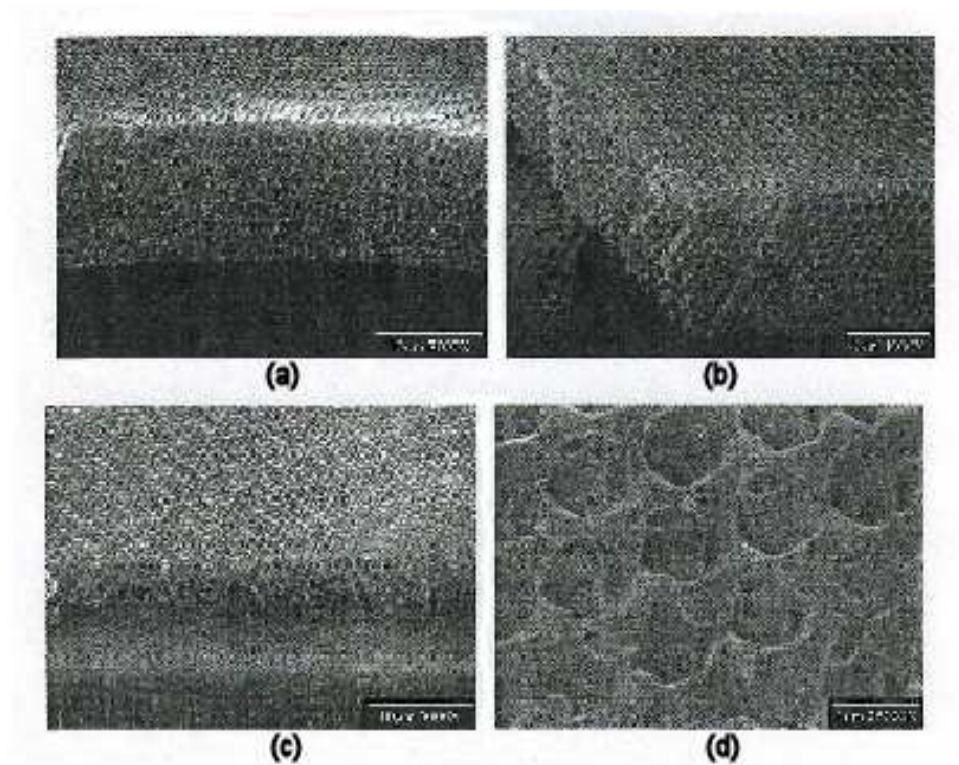
Figure 4.36: SEM images of FCC structure created in SU-8 by Hybrid Technologies using holographic process, (a), (b), (c), and (d) are different views and magnifications of a sample PhC they fabricated [3].
