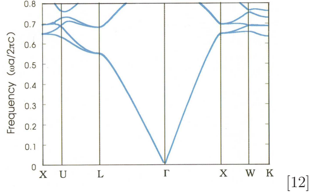
Figure 1.7: Brillouin zone band diagram of a three-dimensional crystal of frequency versus k-space of incorrect geometry and large dielectric contrast of 13 to 1.
