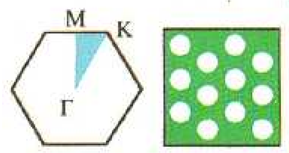
Figure 4.9: Reciprocal lattice space of the crystal; the left picture indicates the wave vector direction observed and the right picture indicates the reciprocal lattice of the two-dimensional triangular structure [12].
