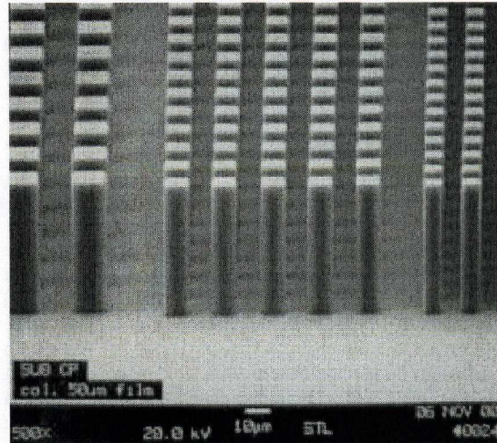
5μm, 10μm and 20μm post arrays in a 50μm thick film.
