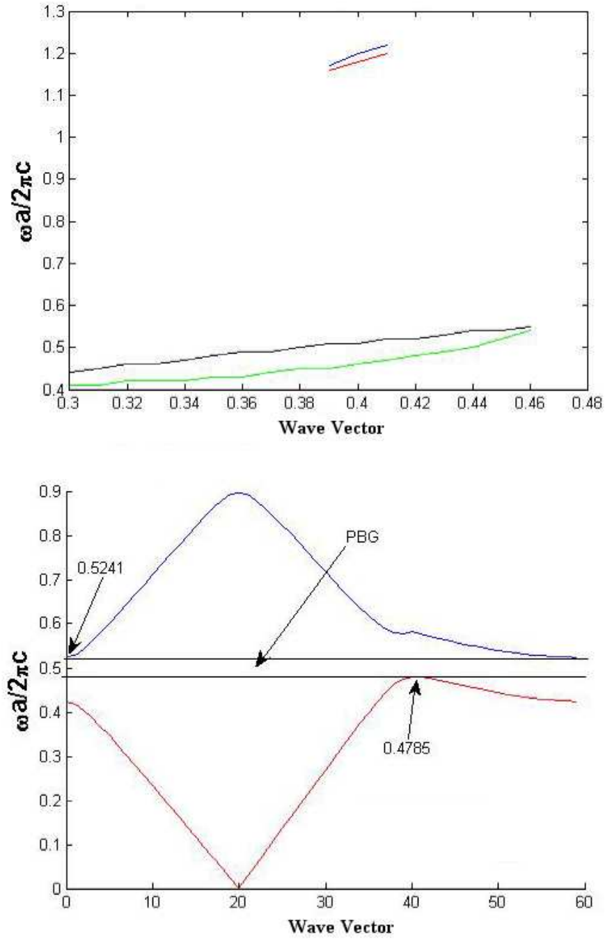
Figure 4.26: Two-dimensional triangular PhC gap map and band diagram for SU-8 negative photo-resist. (a) Gap map with a periodicity of 1\text{ }\mu\text{m} and radius range of 0.3\text{--}0.5\text{ }\mu\text{m} , where the TE field polarization band gap is shown between the green and black lines and the TM field polarization band gap is shown between the red and blue lines. (b) Band diagram of columns of air ( \epsilon = 1 ) in SU-8 ( \epsilon = 2.957 ) for a specific periodicity of 320\text{ nm} and a radius of 134\text{ nm}
