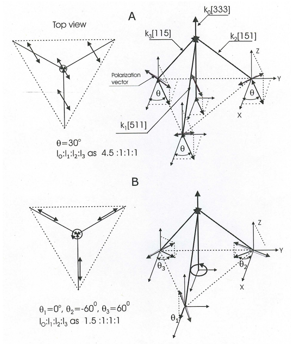
Figure 4.35: Hybrid Technologies laser beam recording geometry for three-dimensional FCC PhC's. (a) Shows the setup for the polarization of all the laser beams projected polarization on the x-y plane forms a 30^\circ angle with the x axis; (b) shows the setup for the polarization of center beam to be circular where as the projection of the side beams (1, 2, and 3) on the x-y plane form a 0^\circ , -60^\circ and 60^\circ angle respectively, with the x axis. [3].
