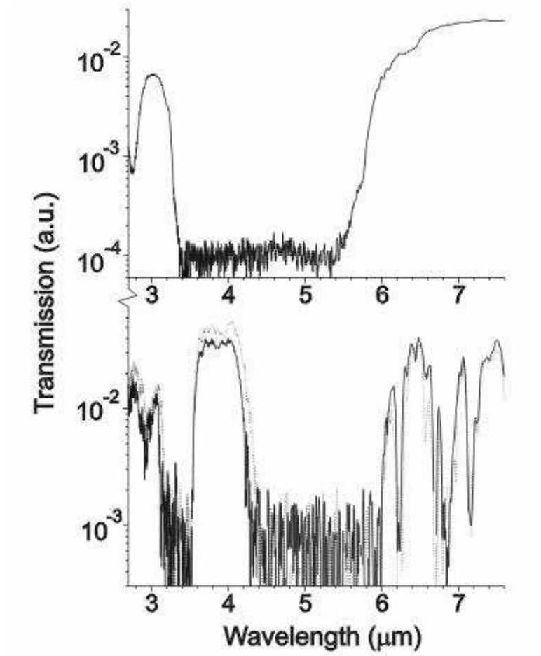
Figure 2.2: (Top) Transmission of H-polarized spectrum prior to infusion of liquid crystal into the PhC of Figure 2.1 and (bottom) after infusion of liquid crystal into the PhC [7].
