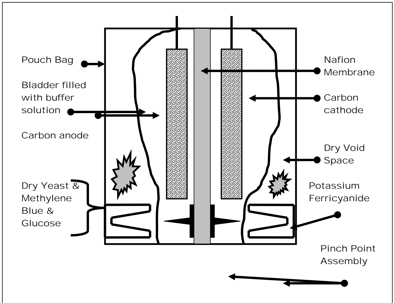
Figure 11. Reserve pouch cell configuration.
