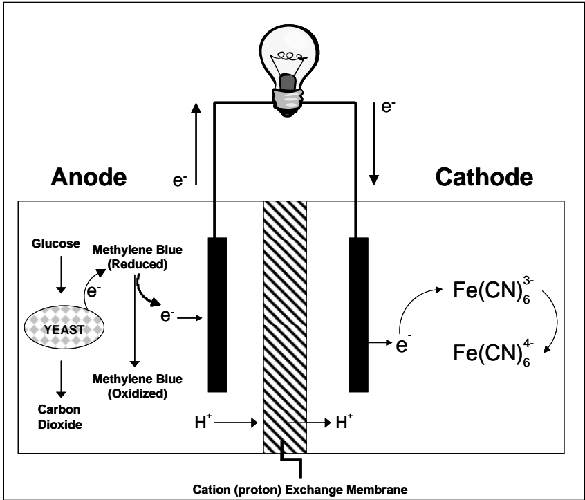
Figure 2. Schematic of the biological fuel cell system.
