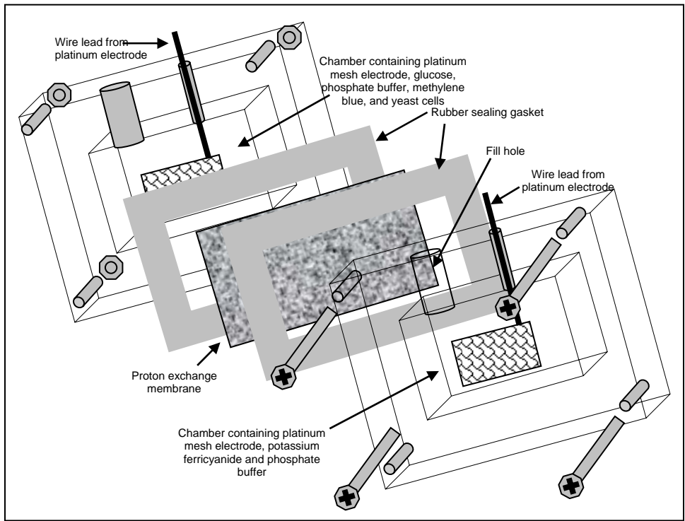
Figure 1. Construction diagram of the plexiglas fuel cell.
