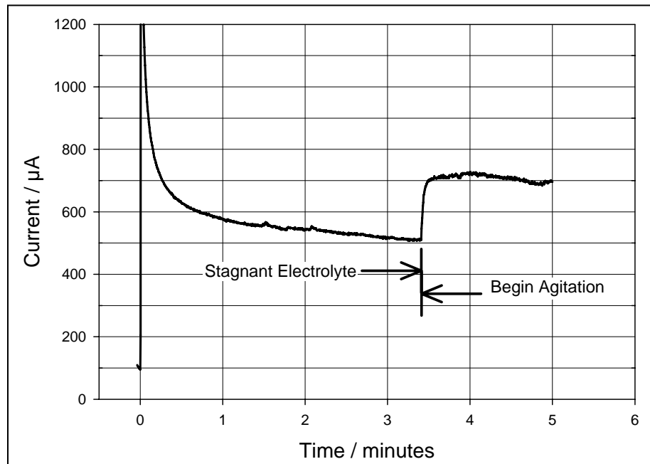
Figure 9. The effect of solution agitation at 45 °C and 0.1 M glucose with 20 mg ml -1 yeast inoculum held at 0.3 V.
