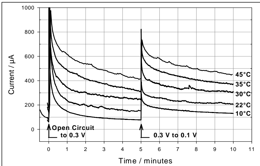
Figure 6. Electrical current produced as a function of temperature with 20 \text{ mg ml}^{-1} of yeast inoculum and 0.1 \text{ M} glucose. (Cell voltage was stepped from OCV to 0.3 \text{ V} for 5 minutes, then stepped to 0.1 \text{ V} for 5 minutes.)
