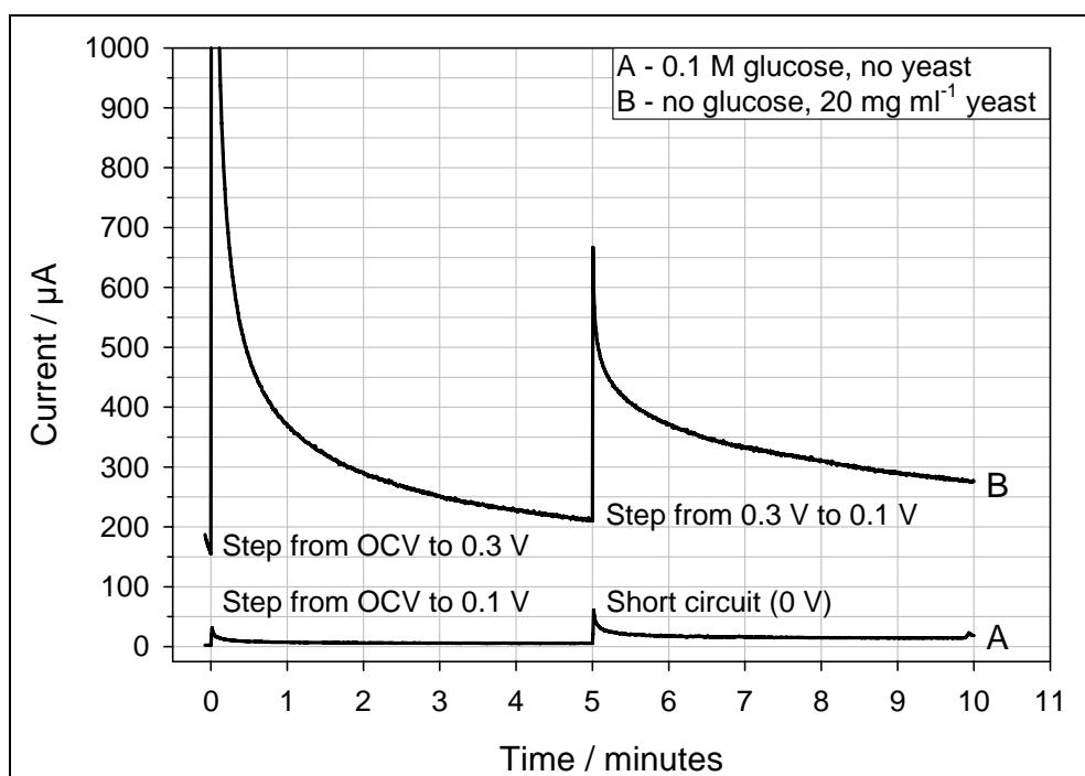
Figure 4. Fuel cell current over time for a complete cell without yeast (A), and for a cell with yeast but without any added glucose (B).
