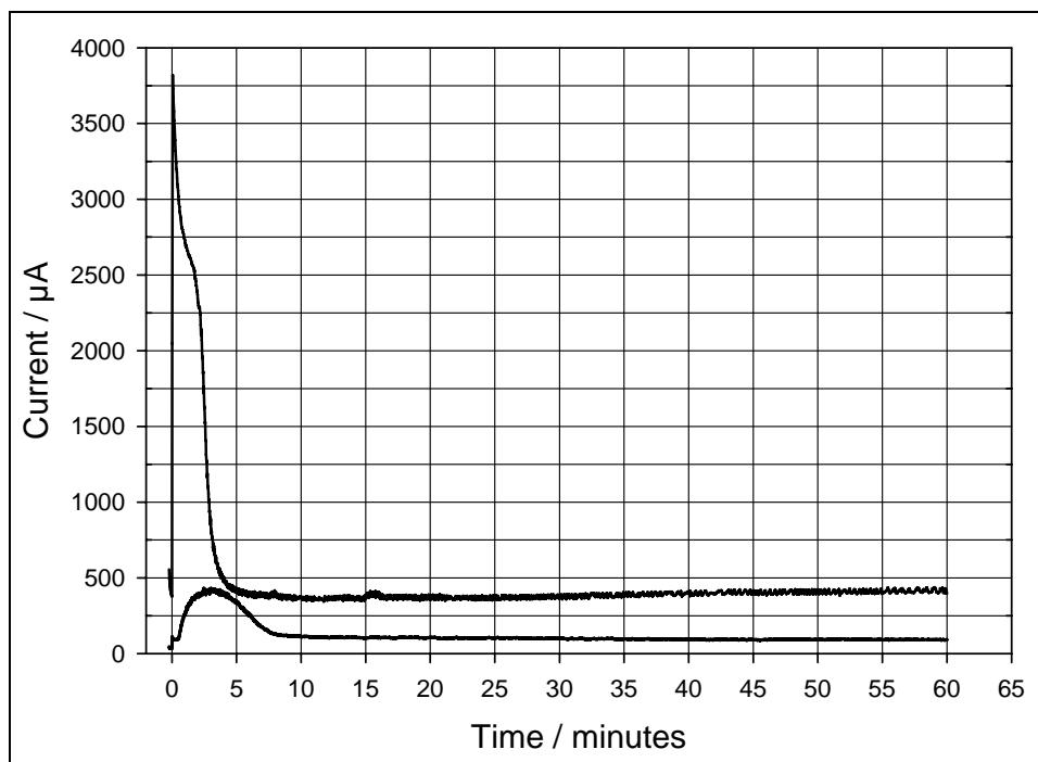
Figure 10. Comparison of the effect of oxygen-saturated (lower trace) and anoxic (upper trace) solutions on current at 45 °C and 0.1 M glucose with 20 mg ml -1 yeast inoculum held at 0.3 V for 1 hour.
