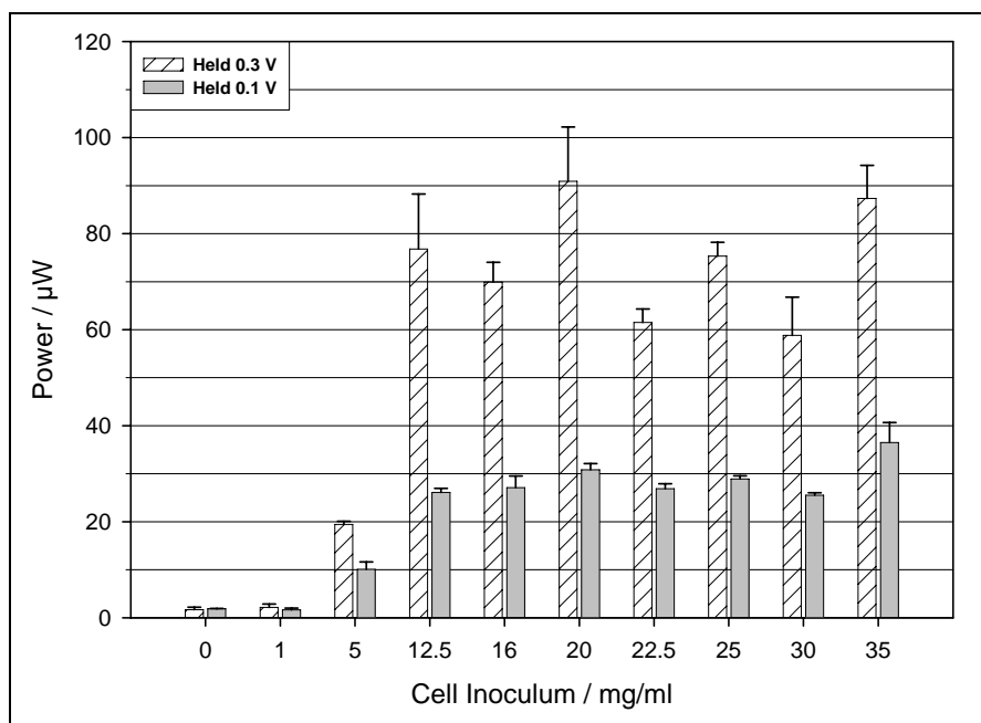
Figure 5. Electrical power generated as a function of concentration of yeast inoculum at 30 \text{ }^\circ\text{C} and 0.1 \text{ M} glucose. (Cell voltage was stepped from OCV to 0.3 \text{ V} for 5 minutes, then stepped to 0.1 \text{ V} for 5 minutes. Average current at the end of 5 minutes was used to calculate power.)
