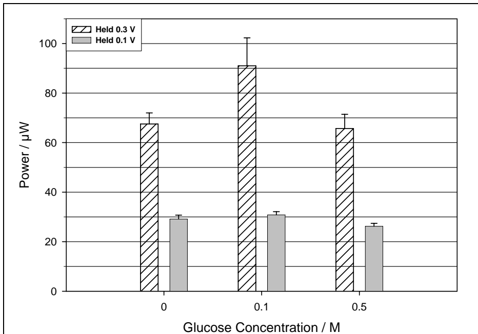
Figure 8. Power generated as a function of glucose concentration for 20 mg ml -1 yeast inoculum at 30 °C.
