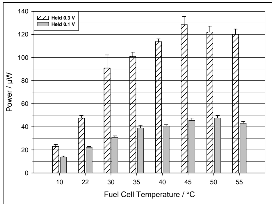
Figure 7. Power generated as a function of cell temperature.
