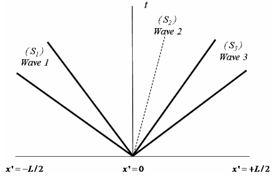
Figure 3.5b. RP Coordinates
