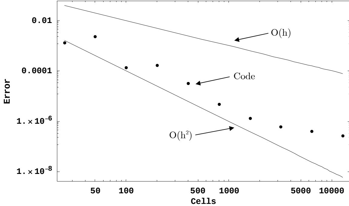
Figure 4.15. Log-Log Plot of Error vs. Number of Cells in Left Star State
