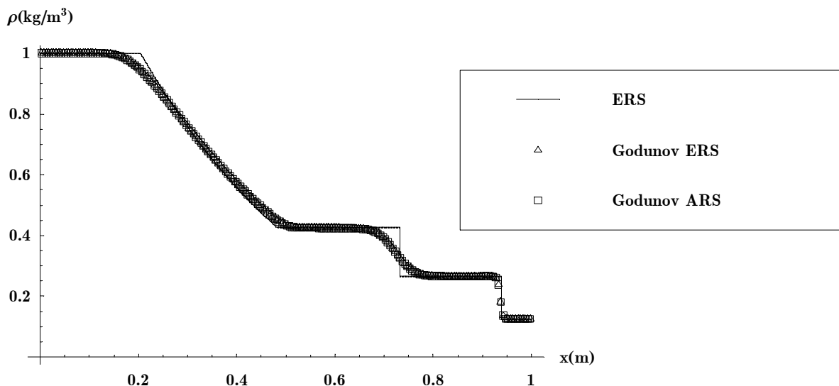
Figure 4.7. Comparison of Godunov's Method Using ERS and ARS
