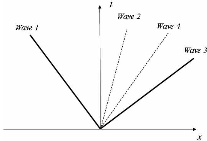
Figure 5.1. Two-Dimensional TVD Flux Limiter Wave Structure
