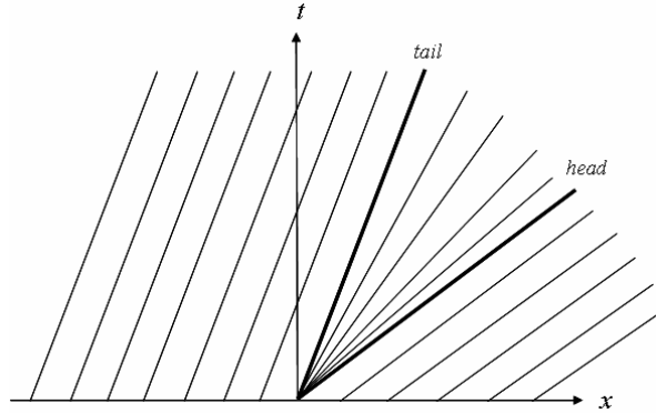
Figure 3.2. Characteristic Field of a Right Moving Rarefaction
