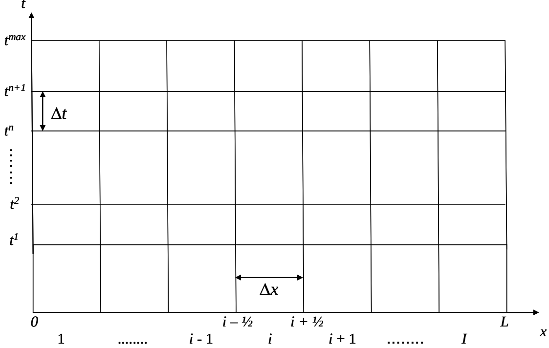
Figure 4.1. Discretized Domain
