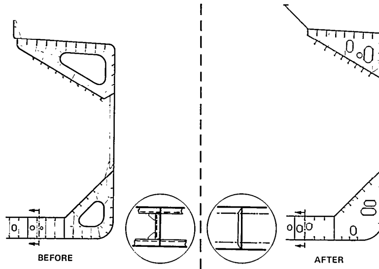
FIG. 16 MIDSHIP SECTION
