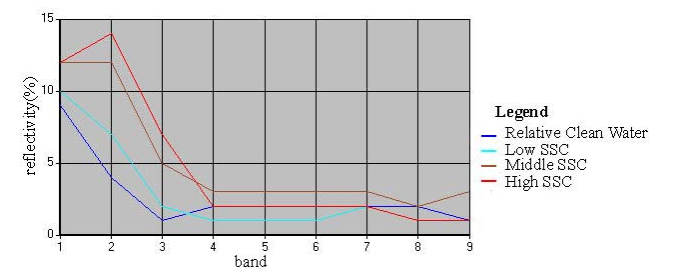
Figure 4. Spectral profile of different SSC water reflectivity
